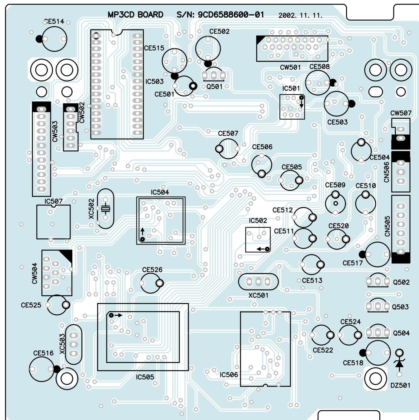
<TOP VIEW>
