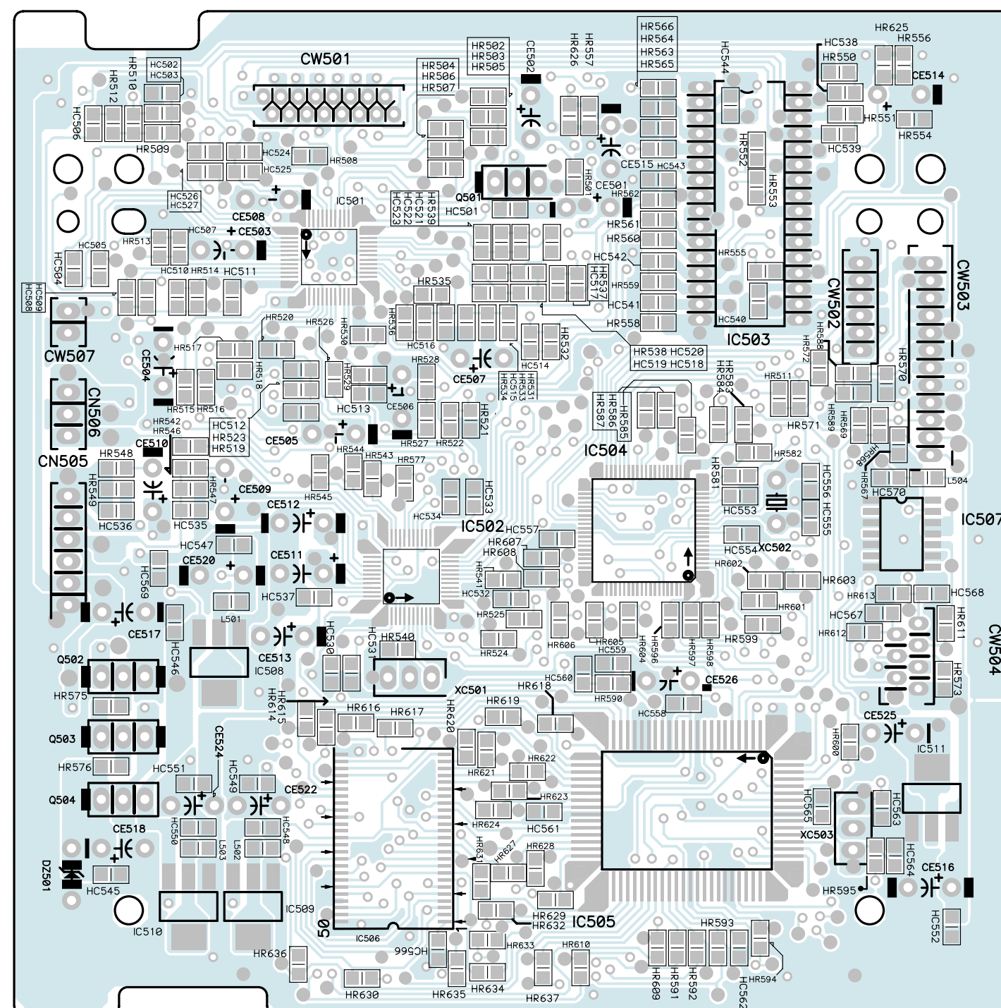
<BOTTOM VIEW>
