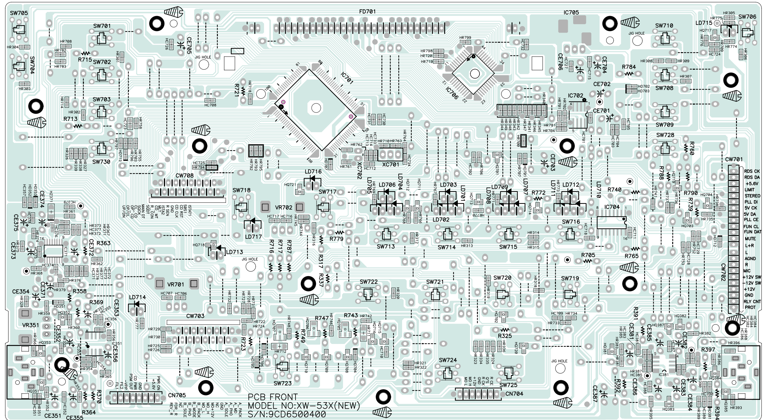
<Bottom View>
