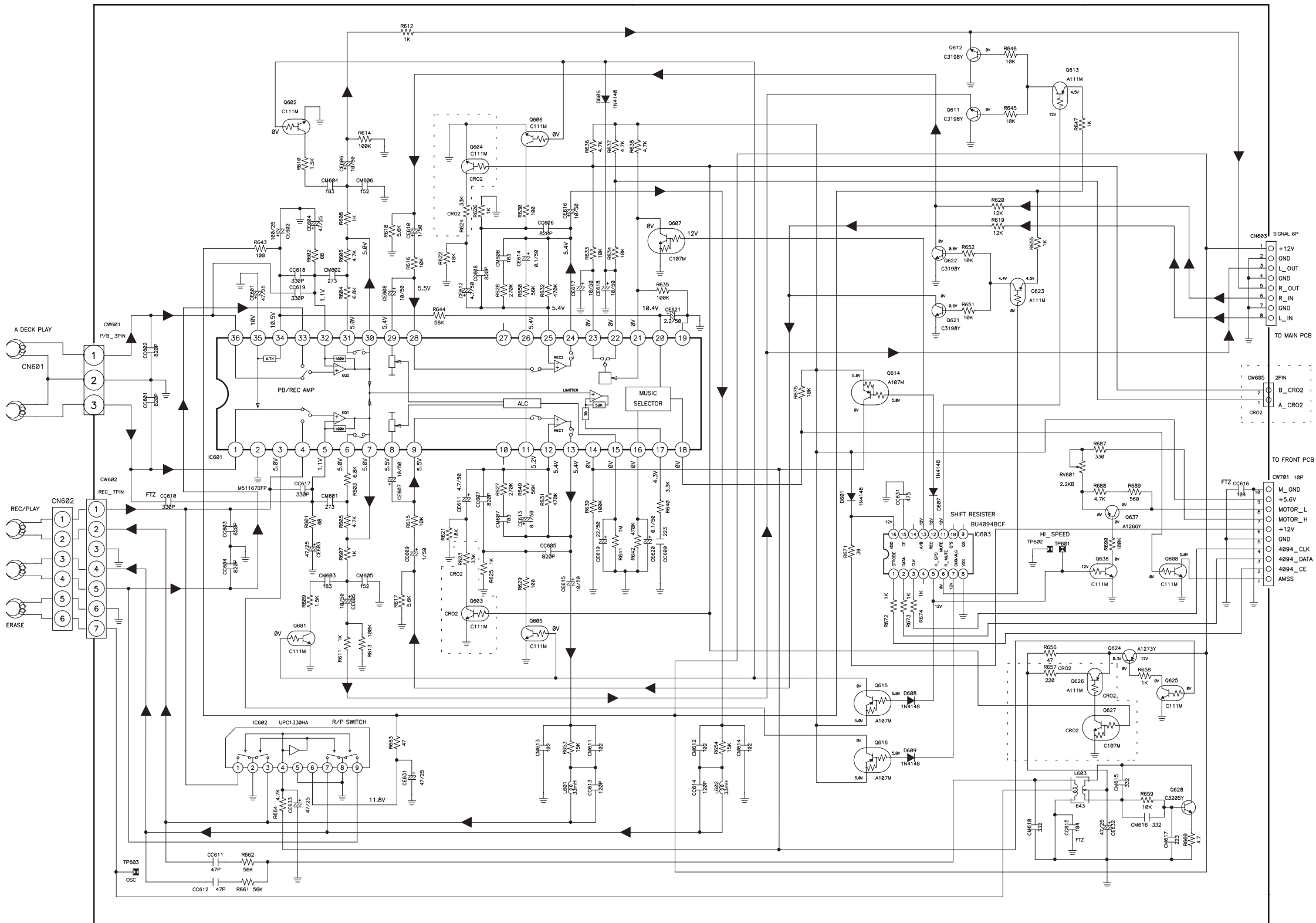
AXL-123DPR TAPE SCHEMATIC DIAGRAM
