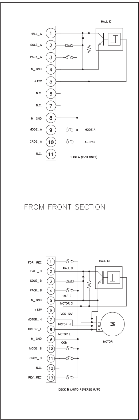
AXL-123DPR TAPE SCHEMATIC DIAGRAM
