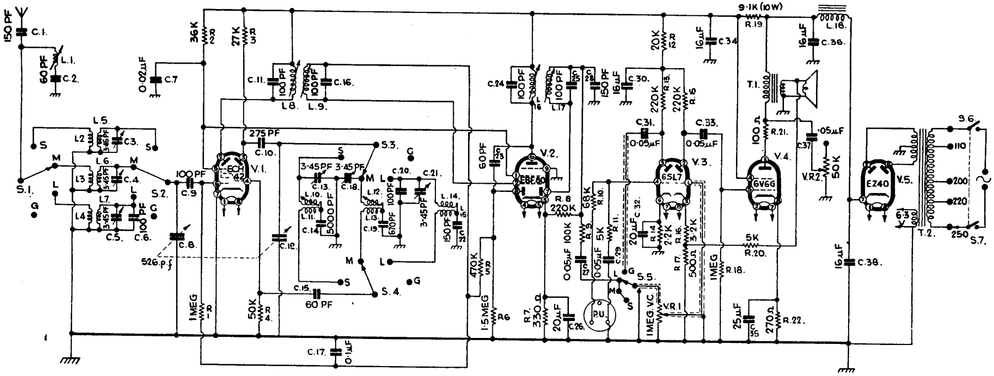
CIRCUIT DIAGRAM—DECCA MODEL 97
