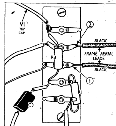
Sketch showing the connecting panel mounted on the side of C27 section of the gang.
