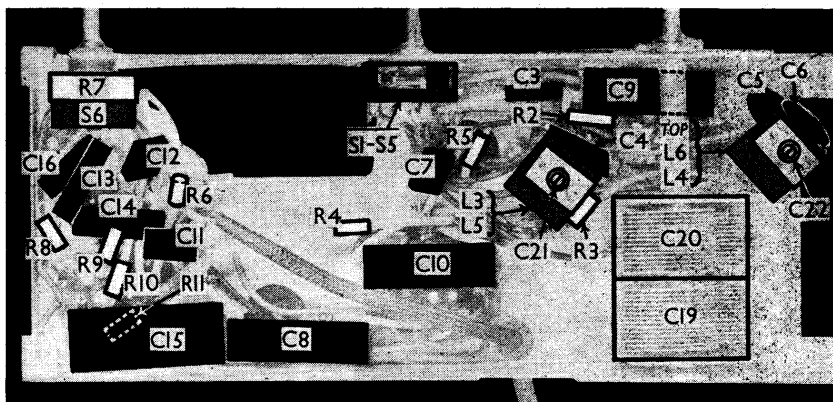
Under-chassis view. A diagram of the SI-S5 switch unit is in column one overleaf.
