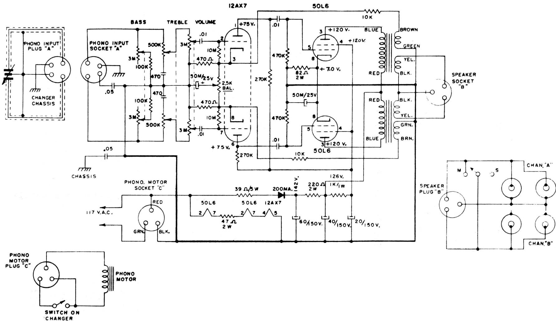
DECCA PHONOGRAPH MODELS DP-630/631 SCHEMATIC DIAGRAM COURTESY OF DECCA DISTRIBUTING
