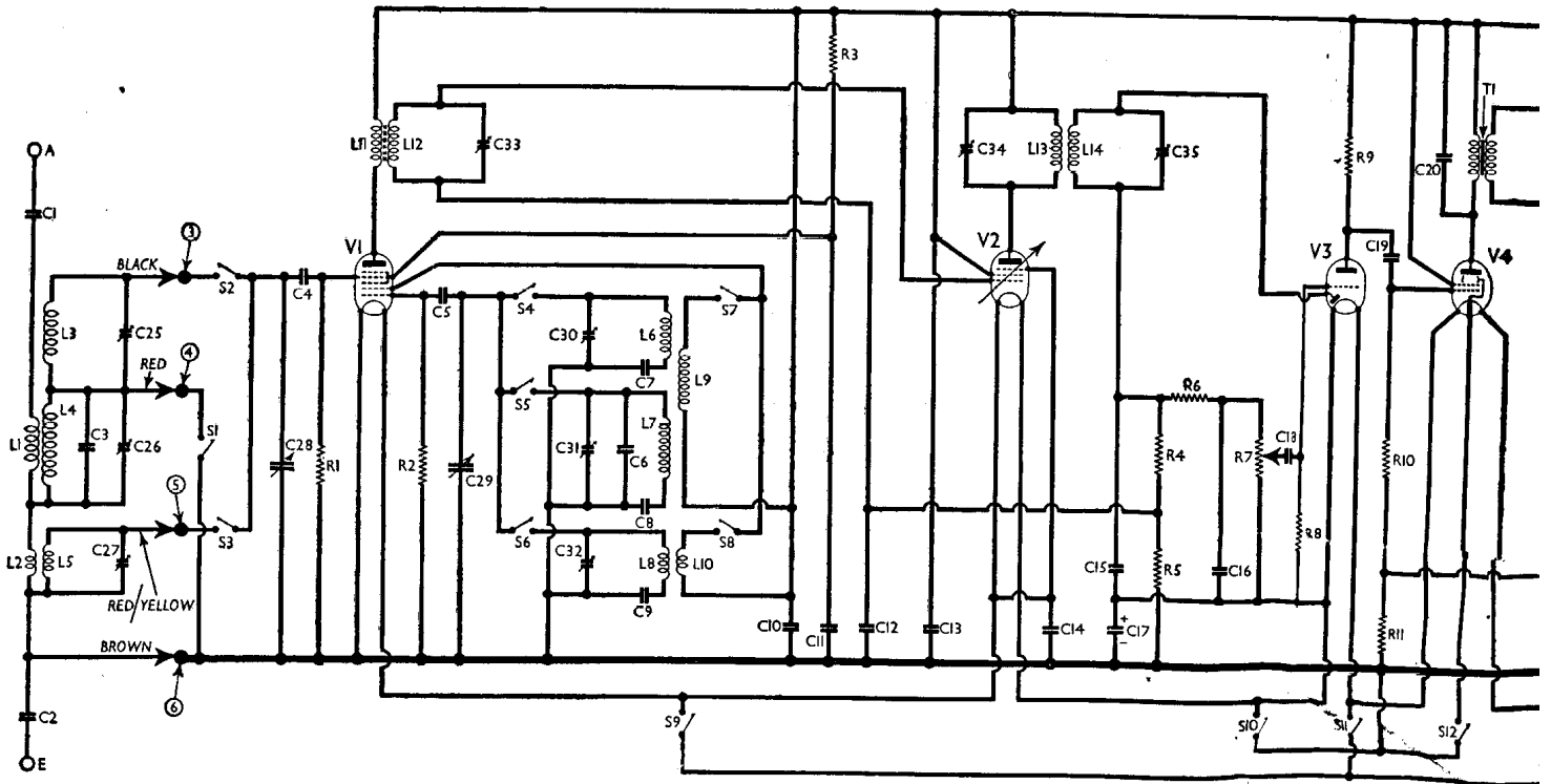
Circuit diagram of the Double Decca model MB5B. Mains input modifications for models MB5A and MB5C are overlaid. N as drawn are, from top to bottom. MW, LW and S.W. A diagram of the battery plug is inset on
