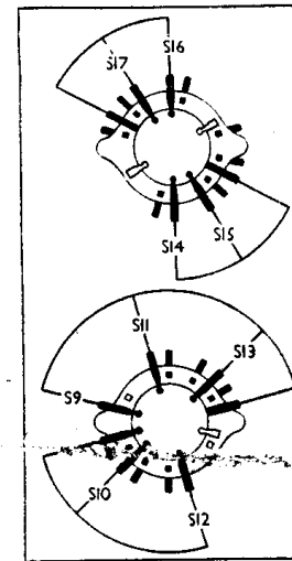
Diagrams of both sides of the S9-S17 unit. Above, the side nearest the control panel; below, the side facing the chassis deck.
