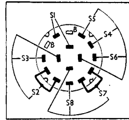
Diagram of the S1-S8 unit, looking at the side facing the chassis deck.
