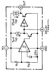
M5128AP (MA: IC351) (SU: IC351) (SU: IC452, 602, 607, 609, 611, 703, 706, 709-712, 716) (RH: IC051, 152)
