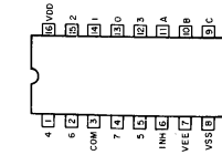
HD14066BP (VV: IC003, 103)
