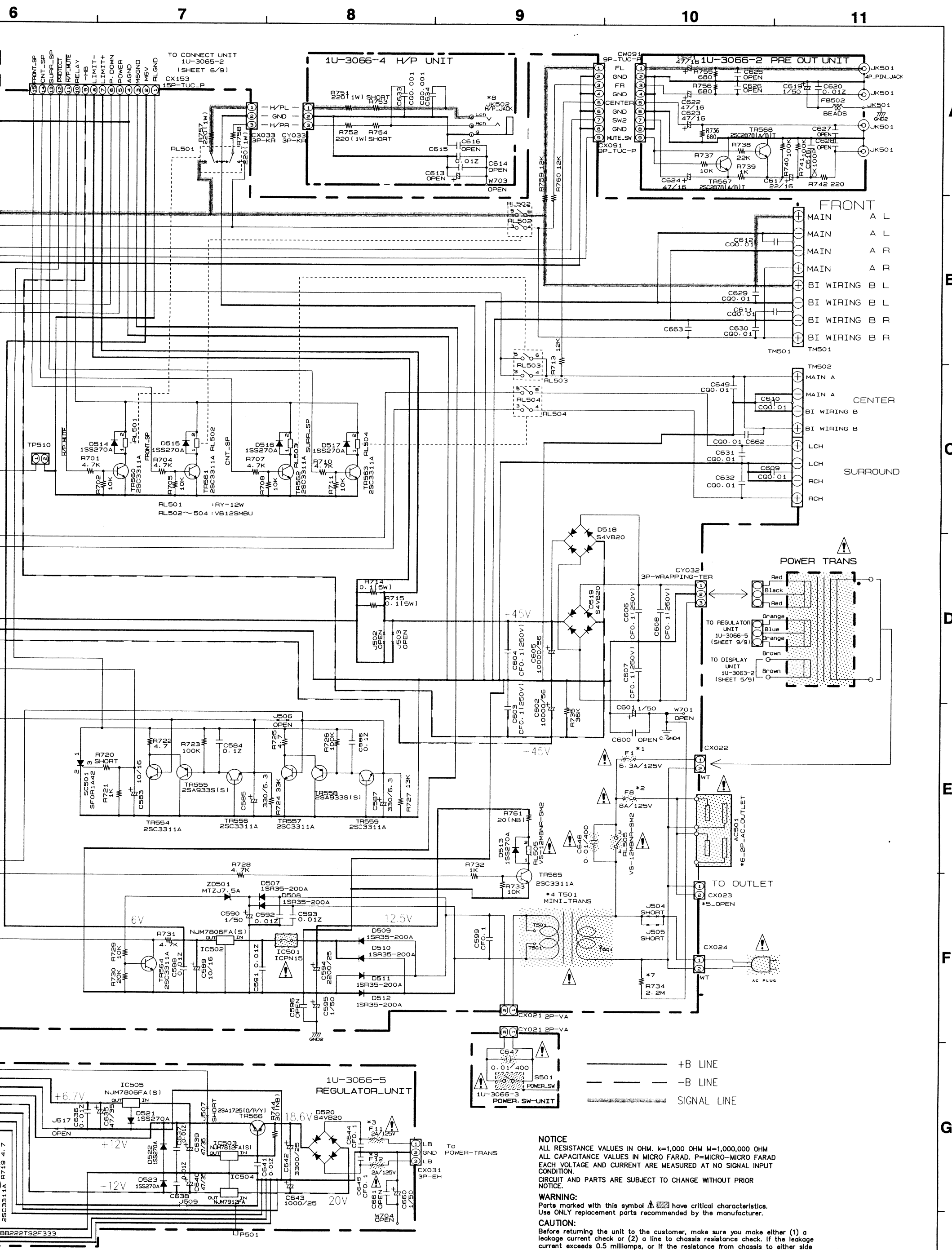
SCHEMATIC DIAGRAM (7/9)
