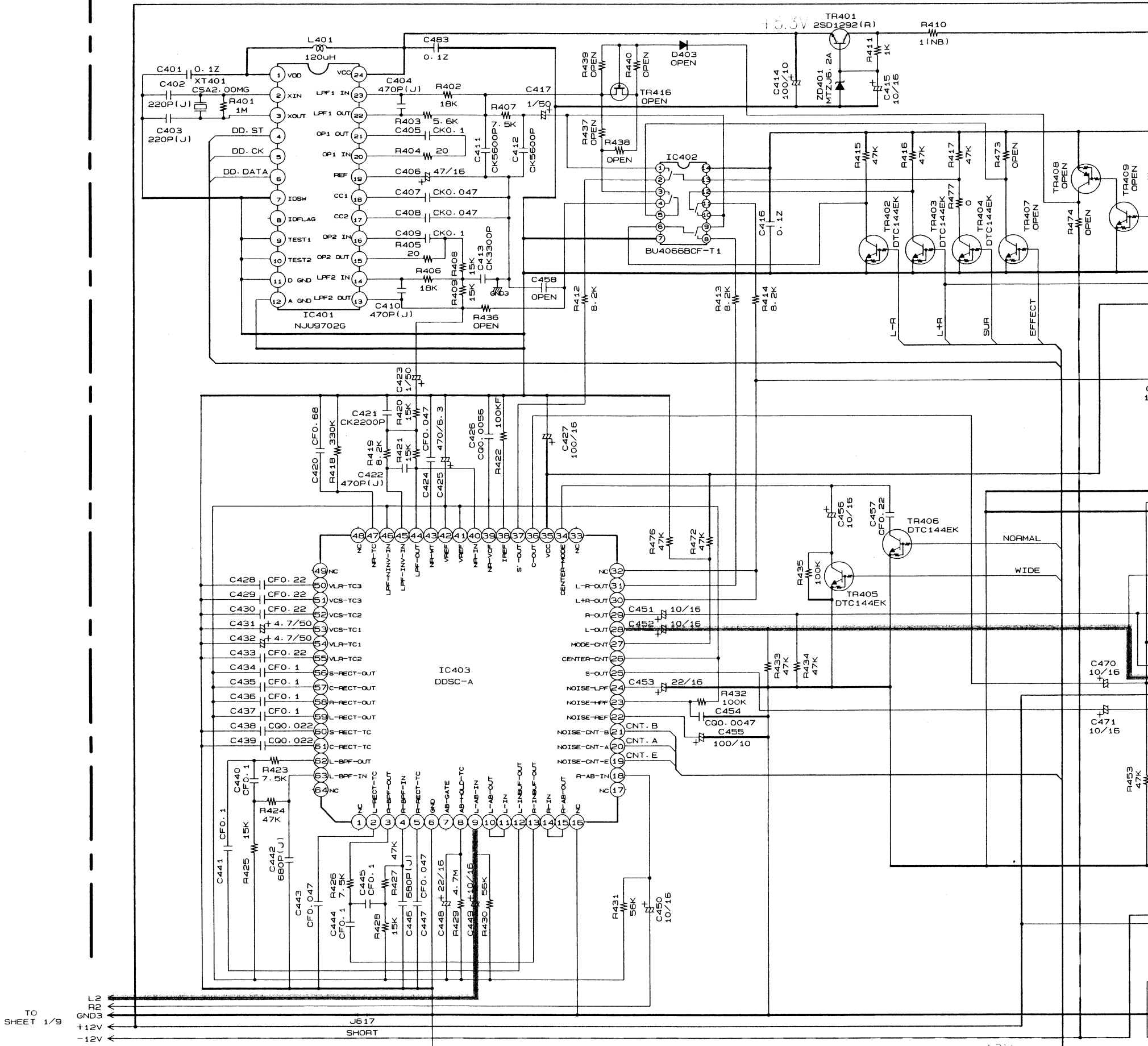
1U-3063-1 INPUT SURROUND UNIT (2/2)
