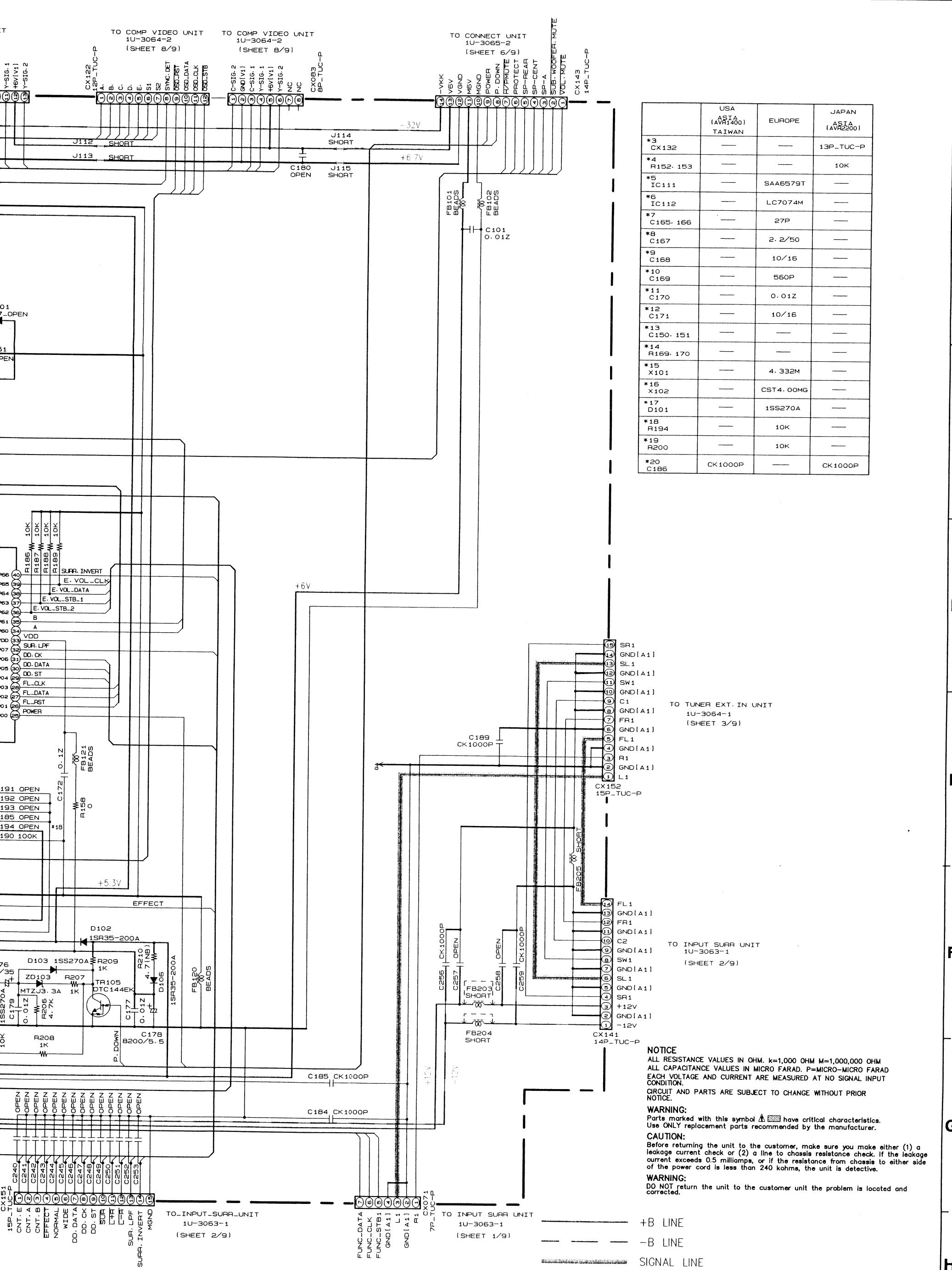
SCHEMATIC DIAGRAM (9/9)
