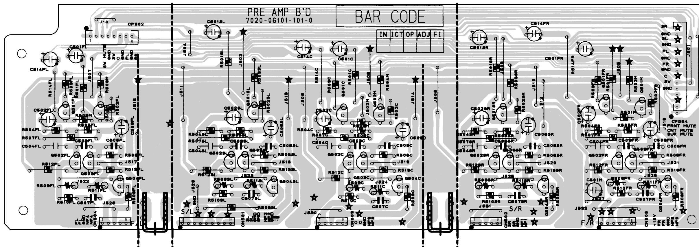
COMPONENT SIDE
