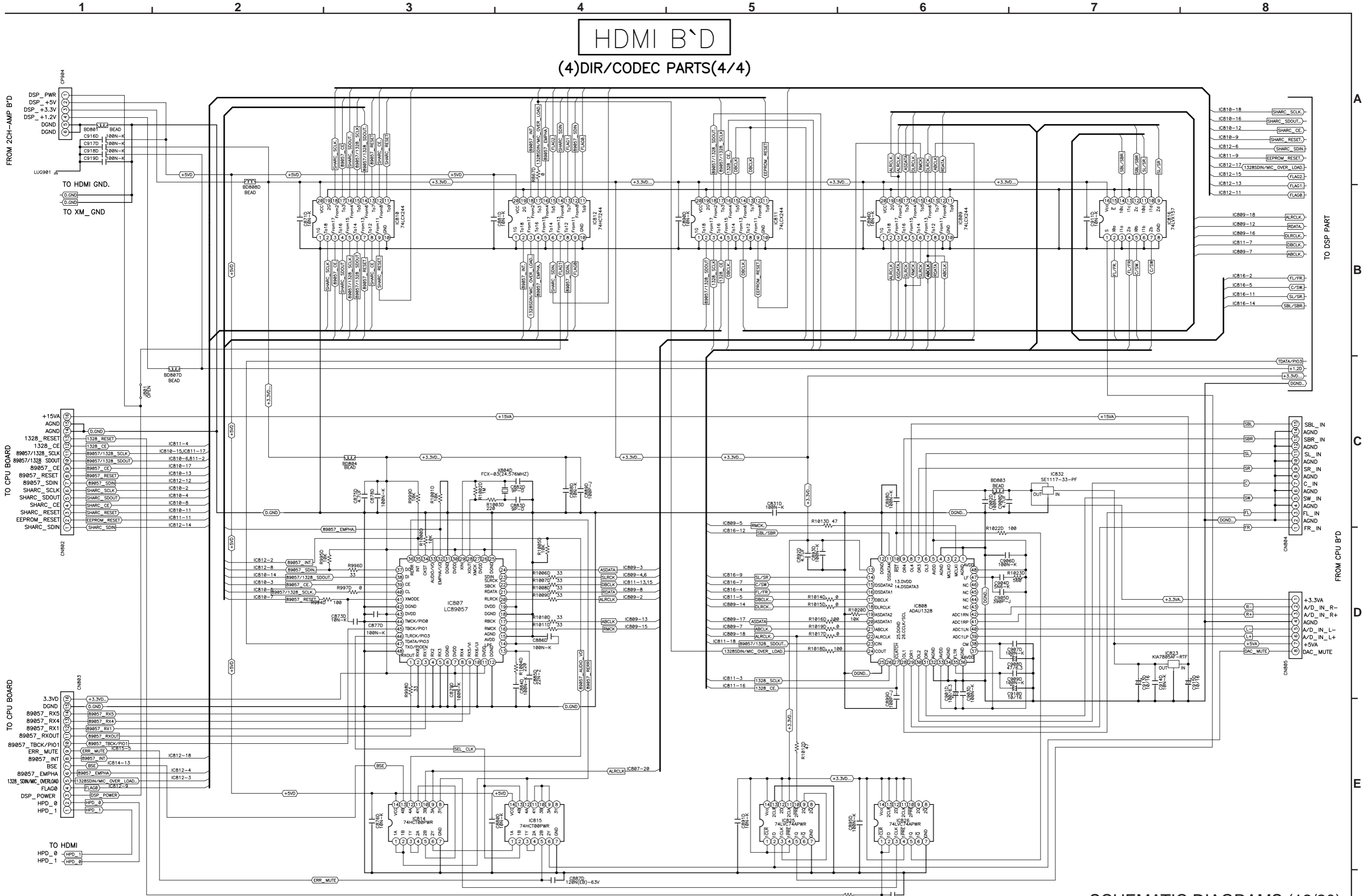
SCHEMATIC DIAGRAMS (12/20) HDMI UNIT (4/4) DIR/CODEC PARTS AVR-1708/1508/688/588/488 AVC-1508
