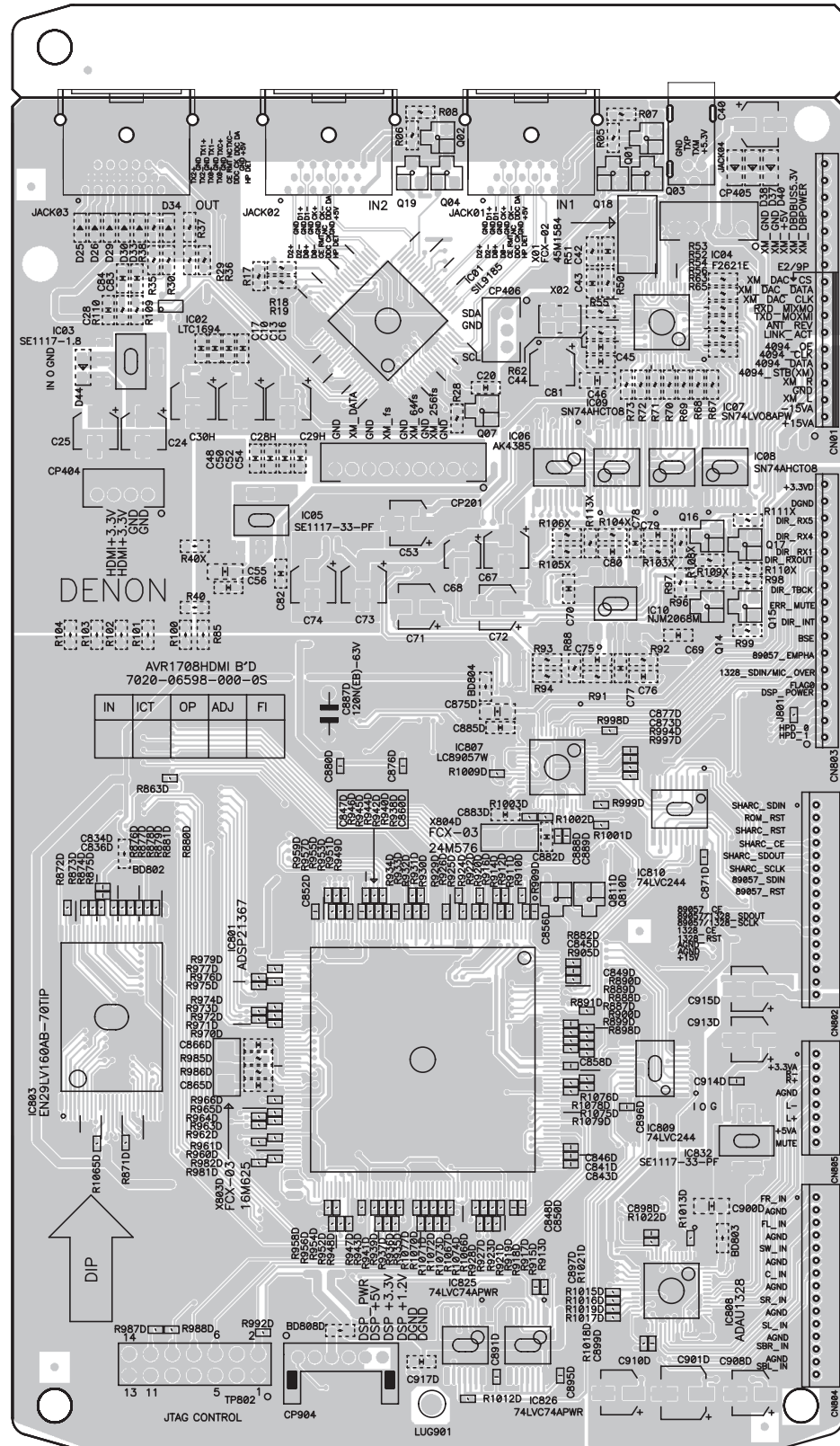
COMPONENT SIDE
