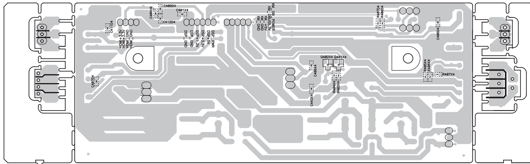
FOIL SIDE
