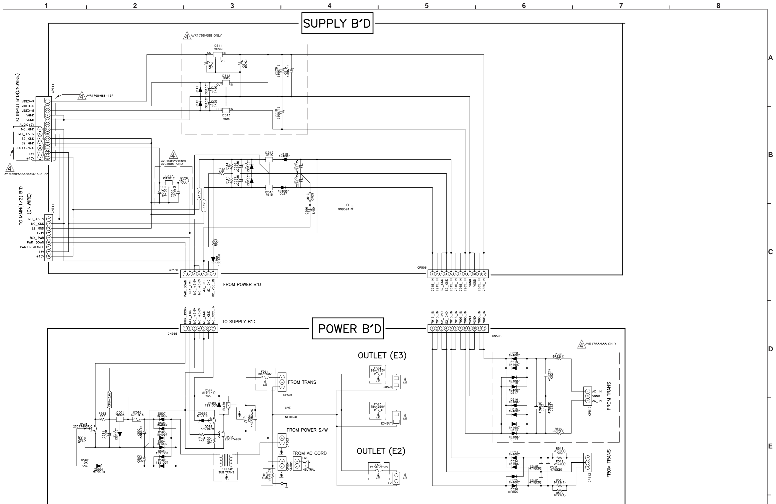
SCHMATIC DIAGRAMS (13/20) SUPPLY UNIT POWER UNIT AVR-1708/1508/688/588/488 AVC-1508
