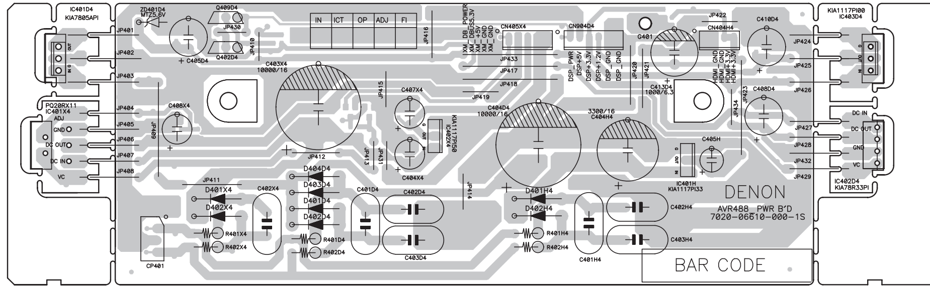
COMPONENT SIDE
