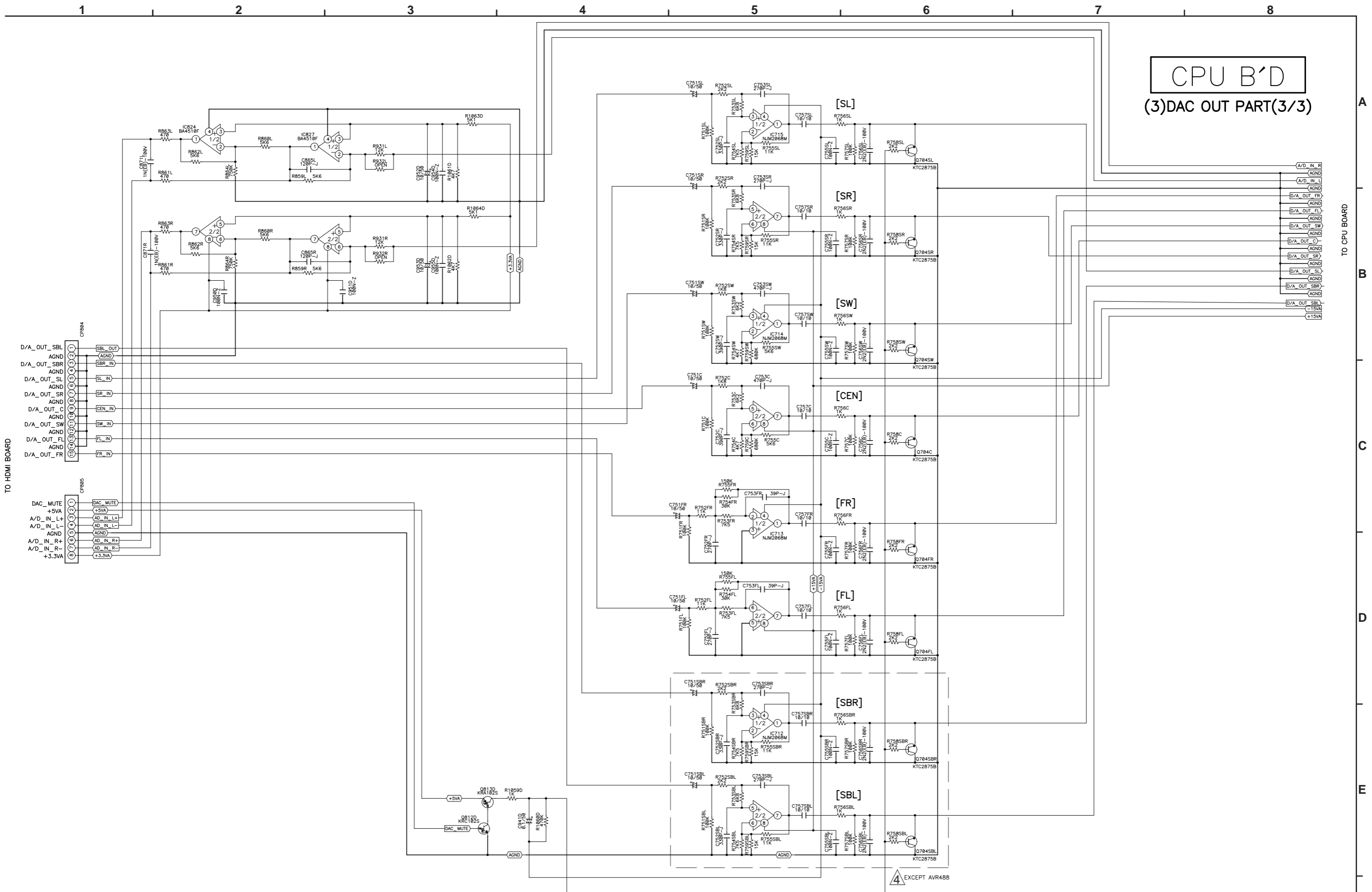
SCHEMATIC DIAGRAMS (6/20) CPU UNIT (3/3) DAC OUT PARTS
