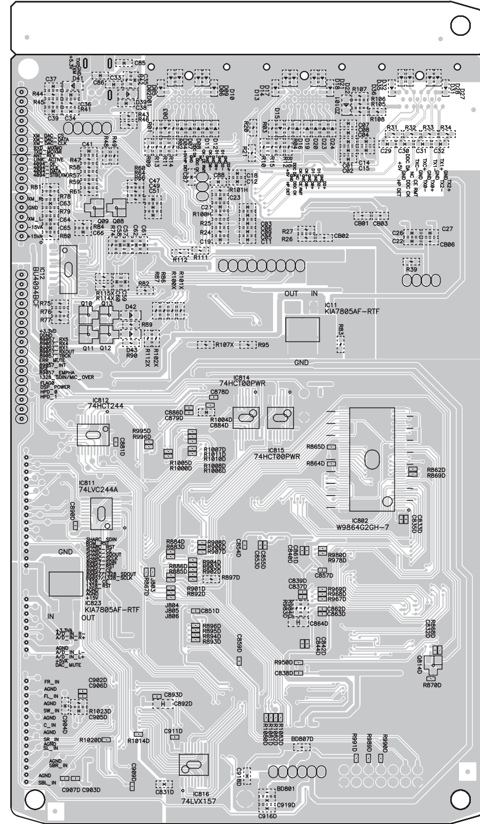
FOIL SIDE
