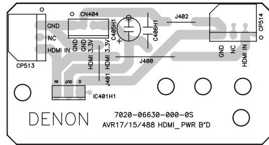
COMPONENT SIDE
