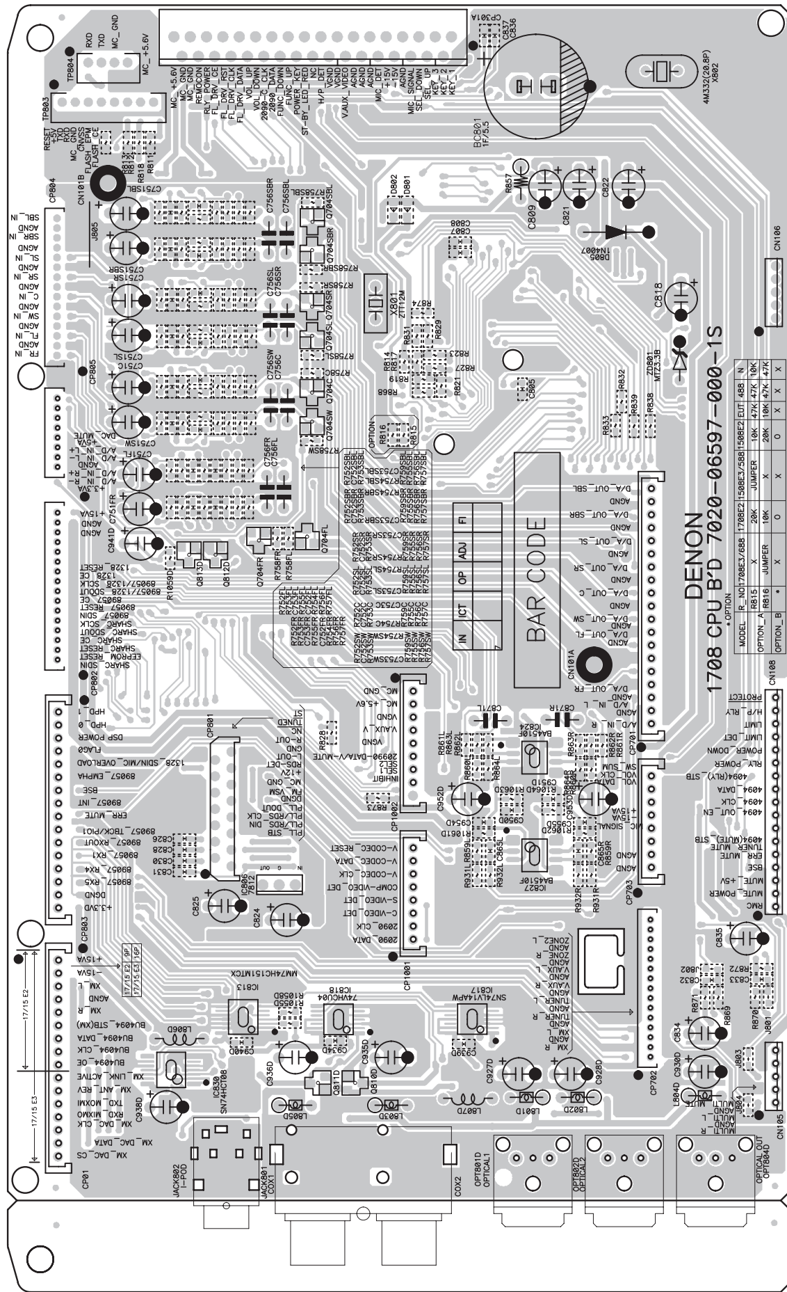
COMPONENT SIDE
