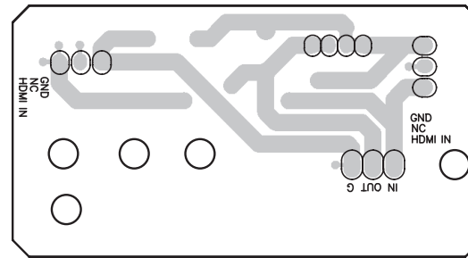
FOIL SIDE
