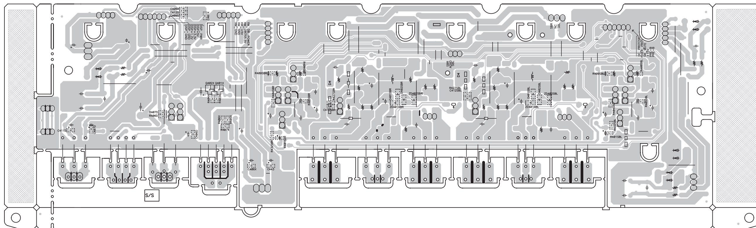
FOIL SIDE
