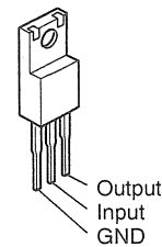
NJM7912FA (RE: IC504)
