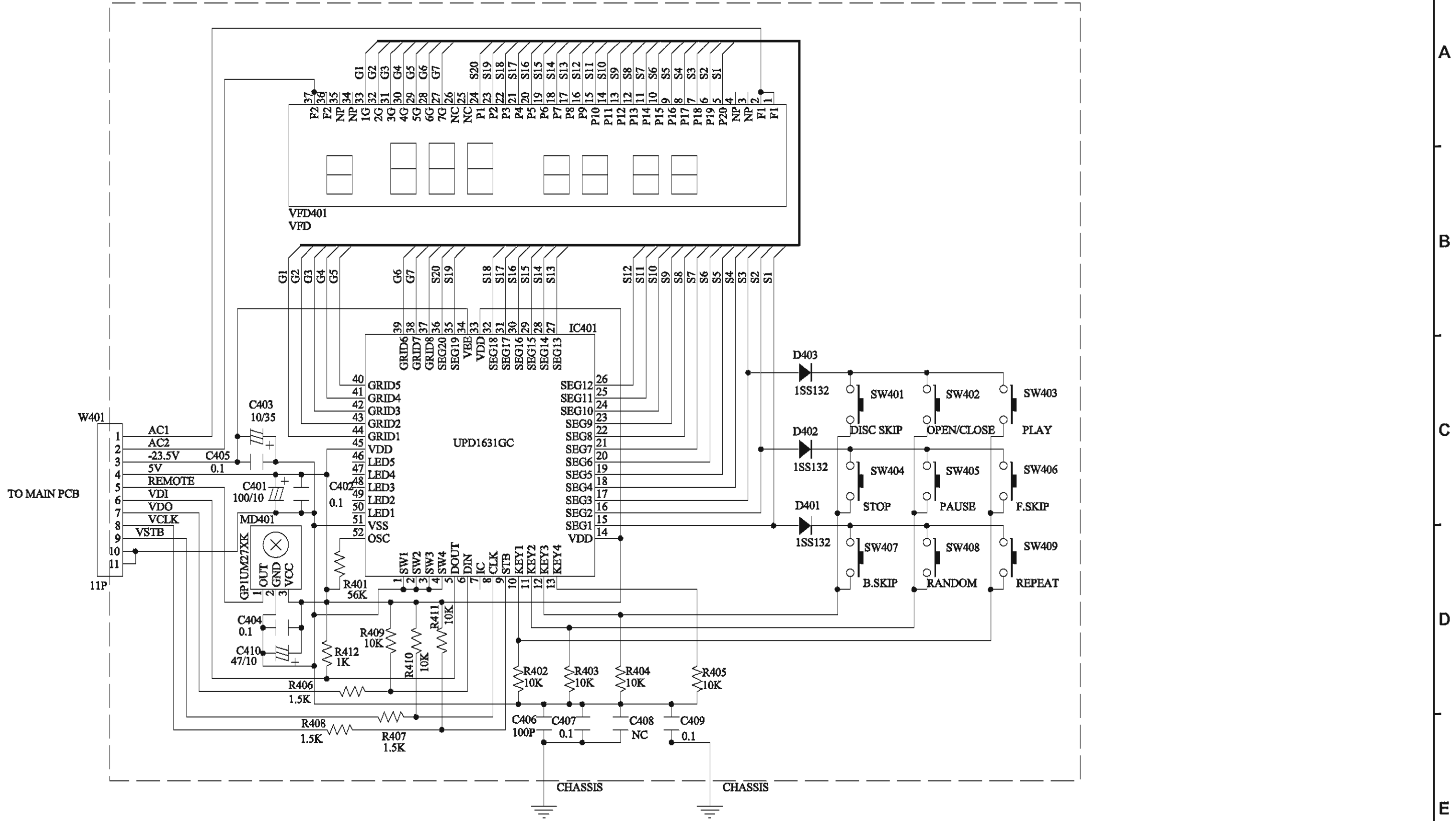
SCHEMATIC DIAGRAMS (3/3) CONTROL UNIT
