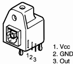
GP1F32R (JACK102,103)
