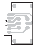
COMPONENT SIDE
