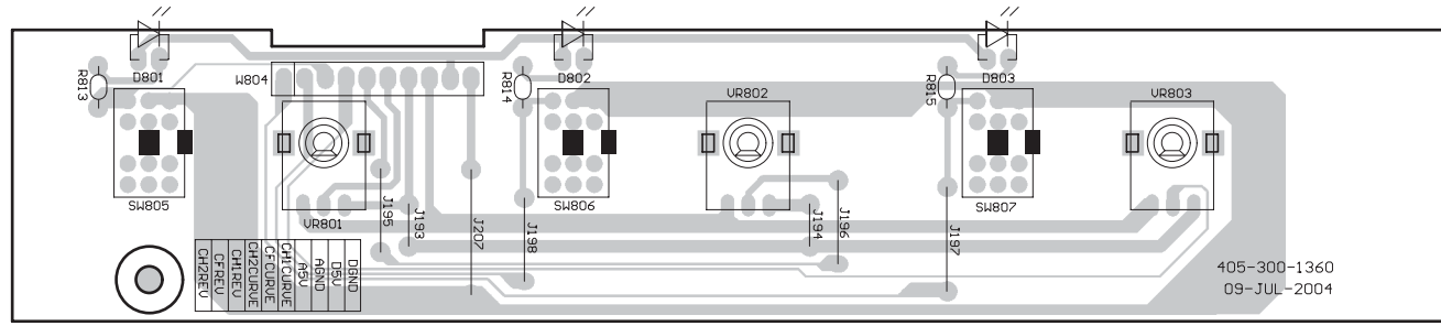
COMPONENT SIDE
