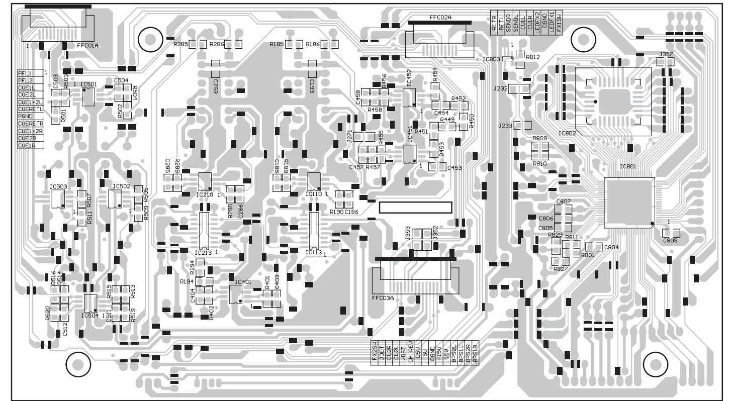
FOIL SIDE
