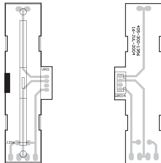
COMPONENT SIDE
