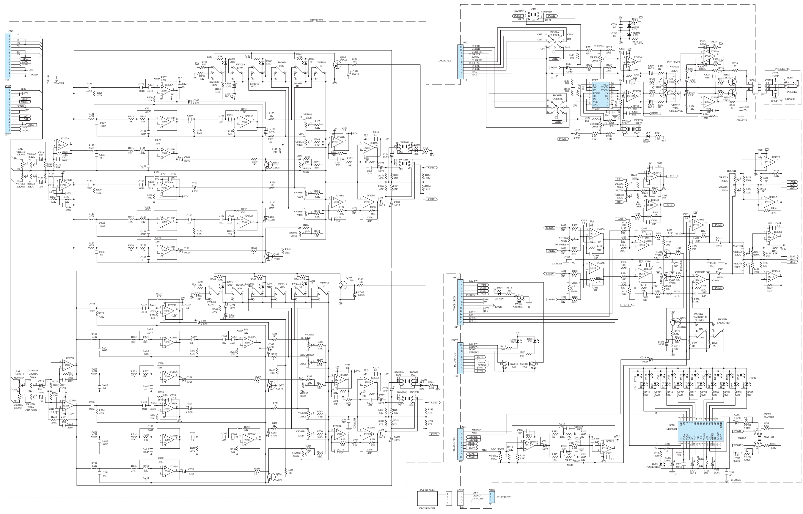
SCHEMATIC DIAGRAMS (1/3) MIXER UNIT PHONE UNIT
