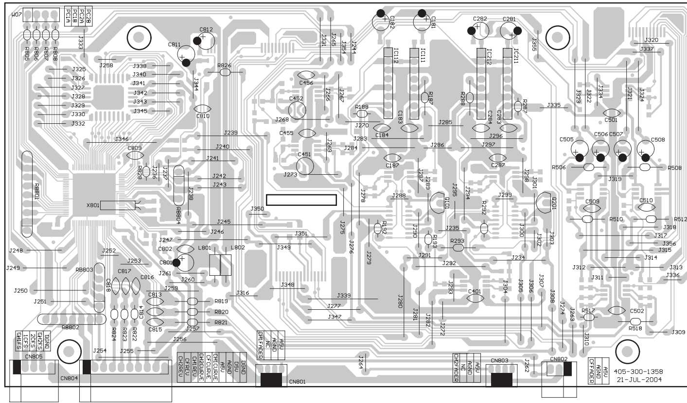
COMPONENT SIDE
