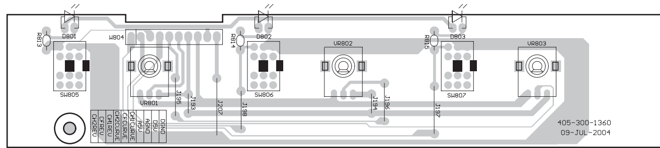
COMPONENT SIDE
