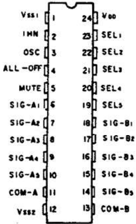
TC9152P (Toshiba)
