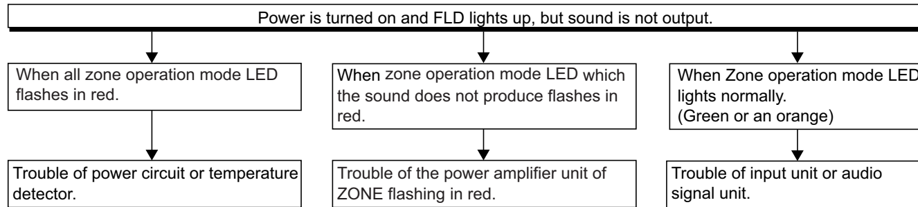
FLOW CHART NO.3
