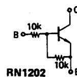
RN1202(10K-10K) NPN RN2202(10K-10K) PNP
