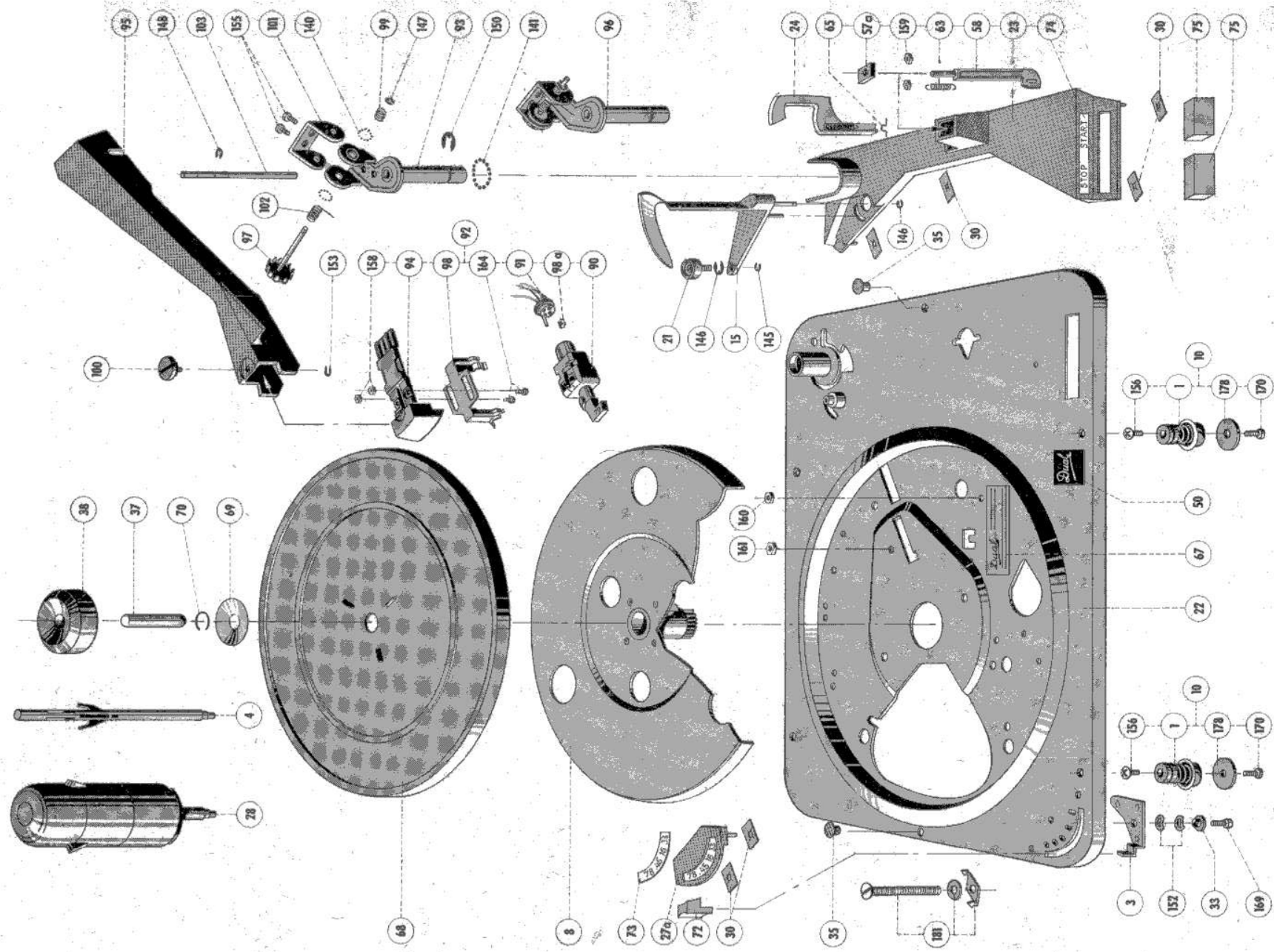
8. Explosive View Fig. 14. parts above chassis
