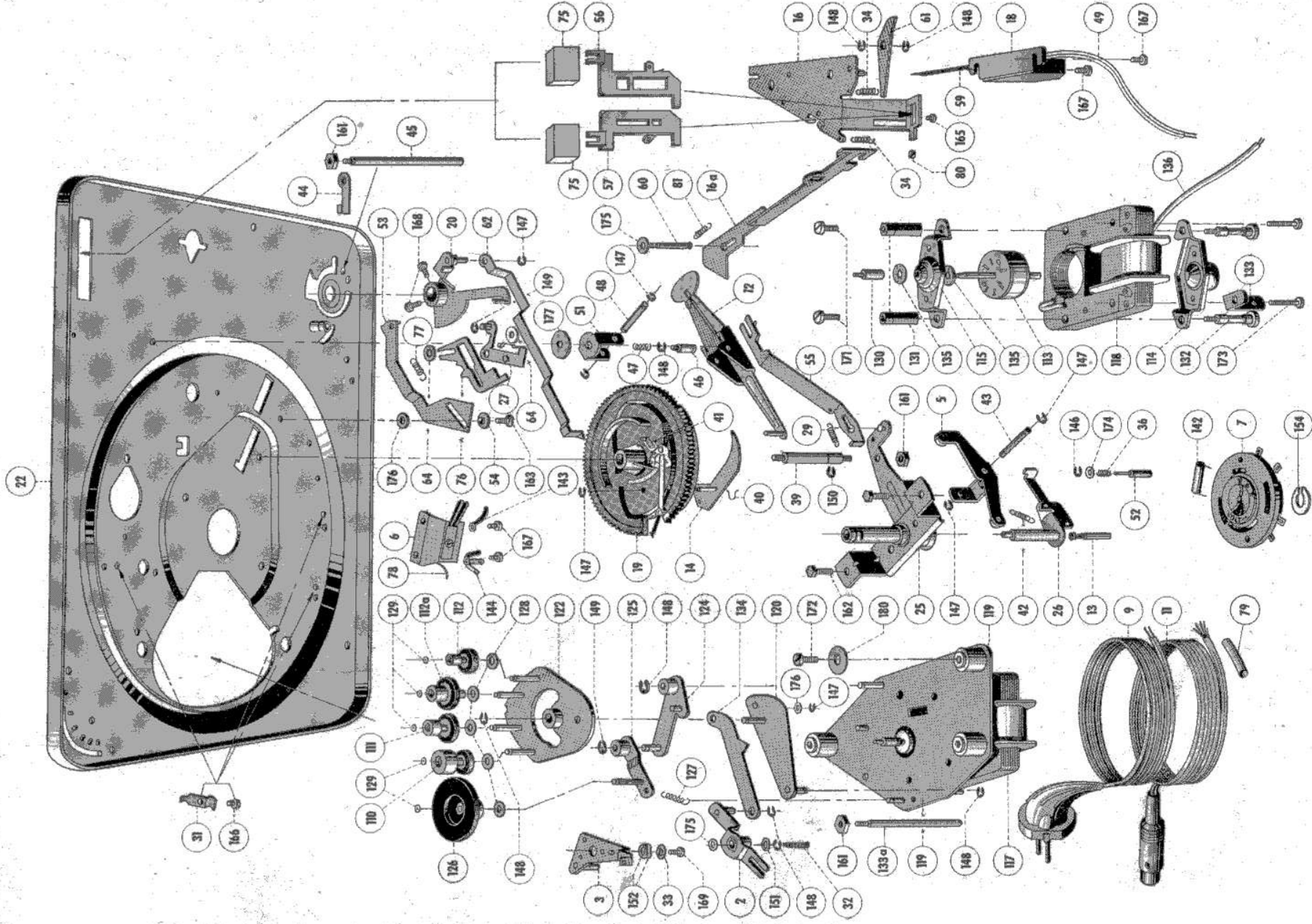
Fig. 15, parts below chassis
