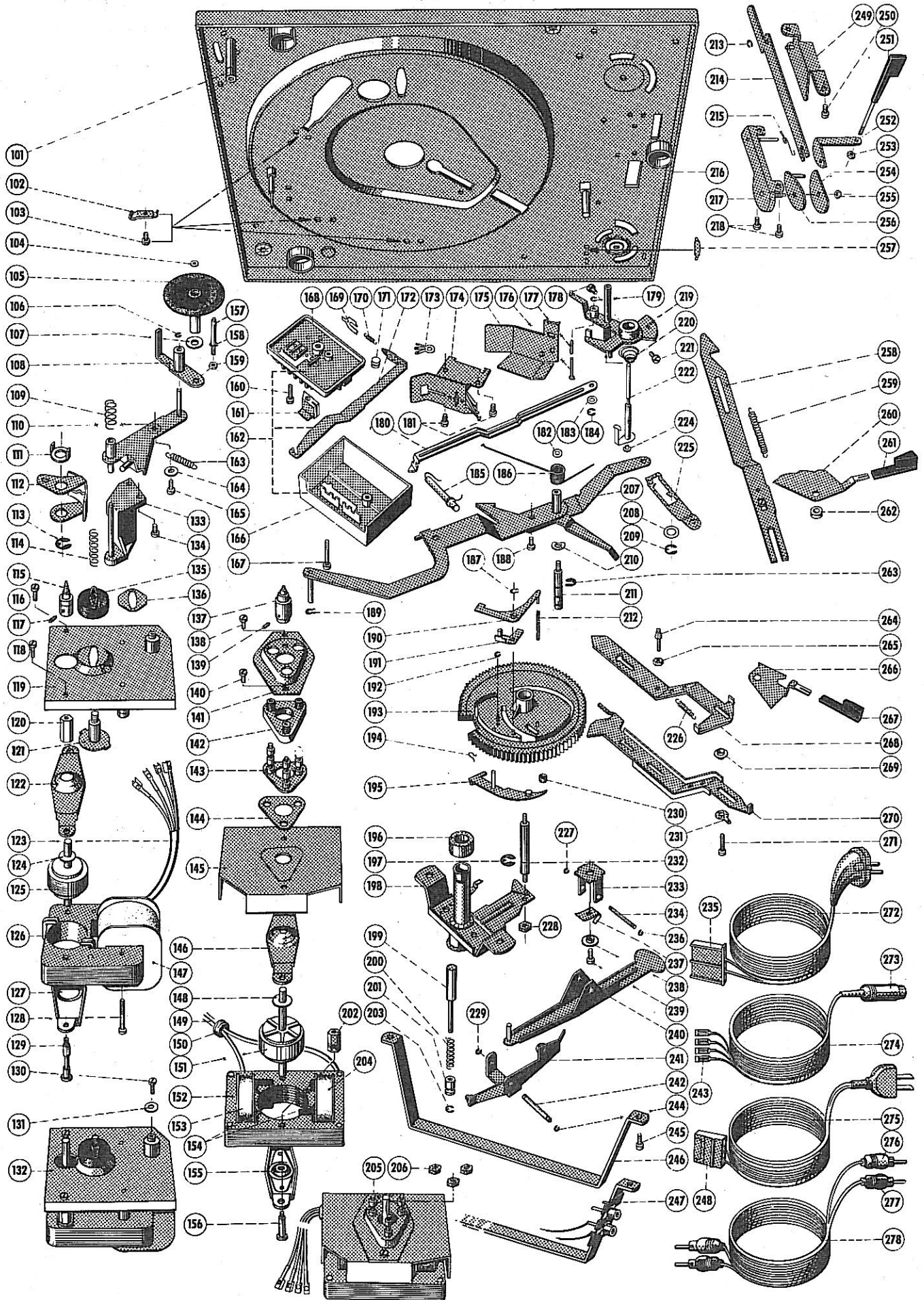
Fig. 2 Exploded view, parts below chassis
