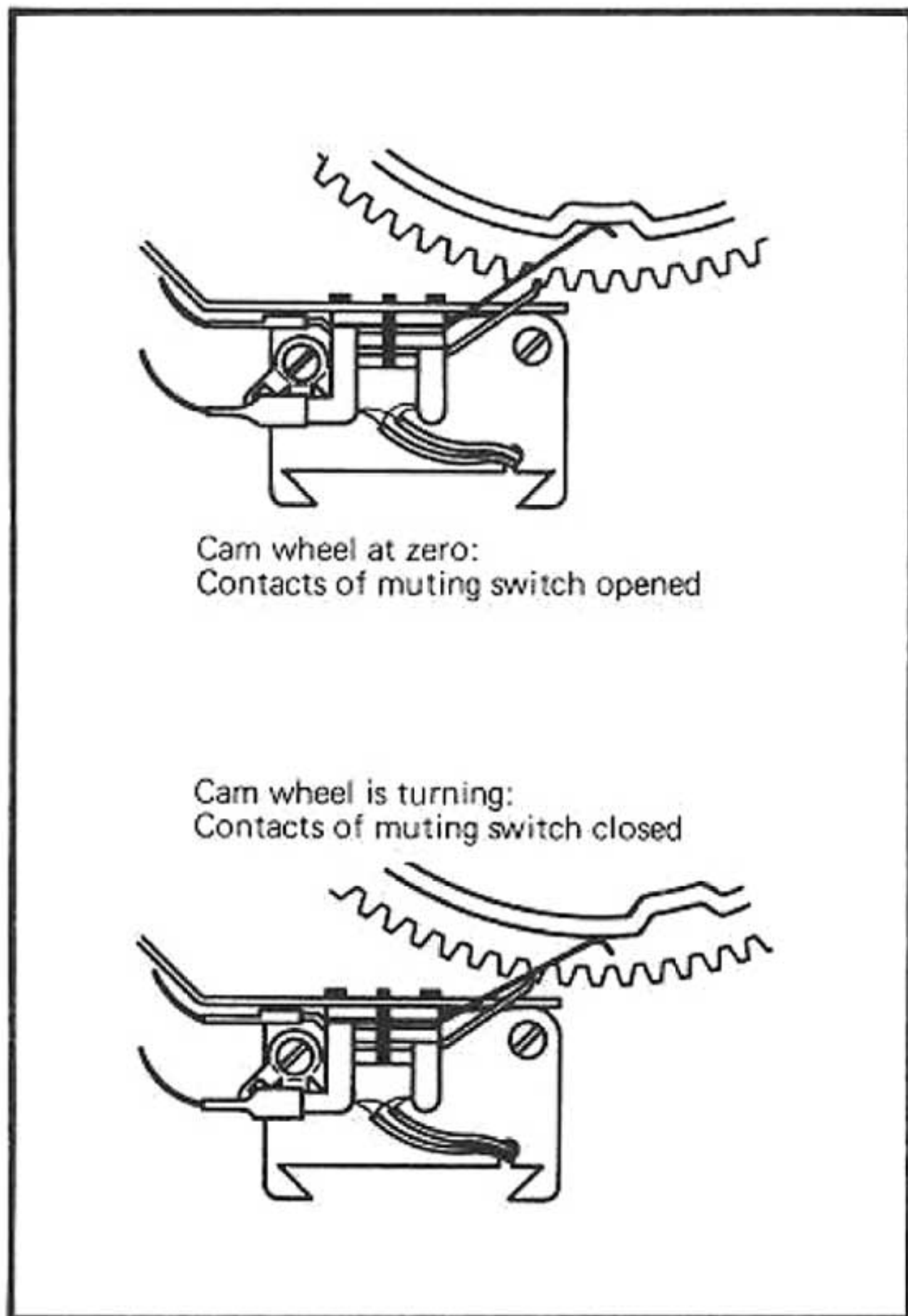
Fig. 14 Muting switch
