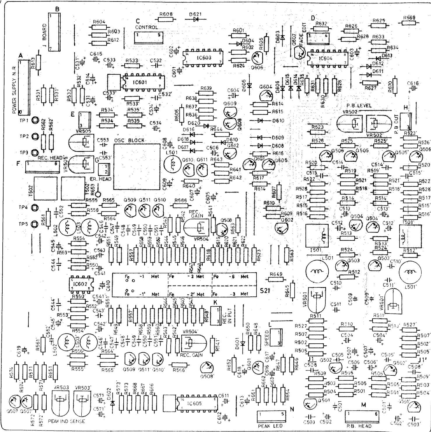
A A.M.P. PARTS LOCATION TOP VIEW
