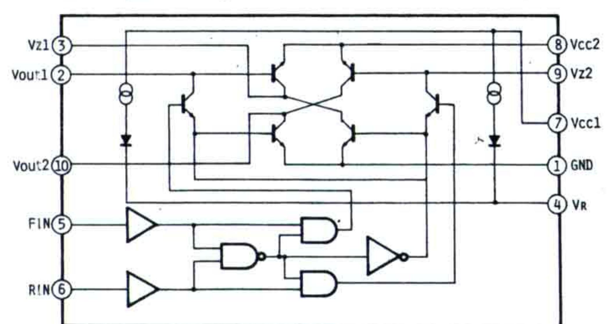
IC900(BA6109)
