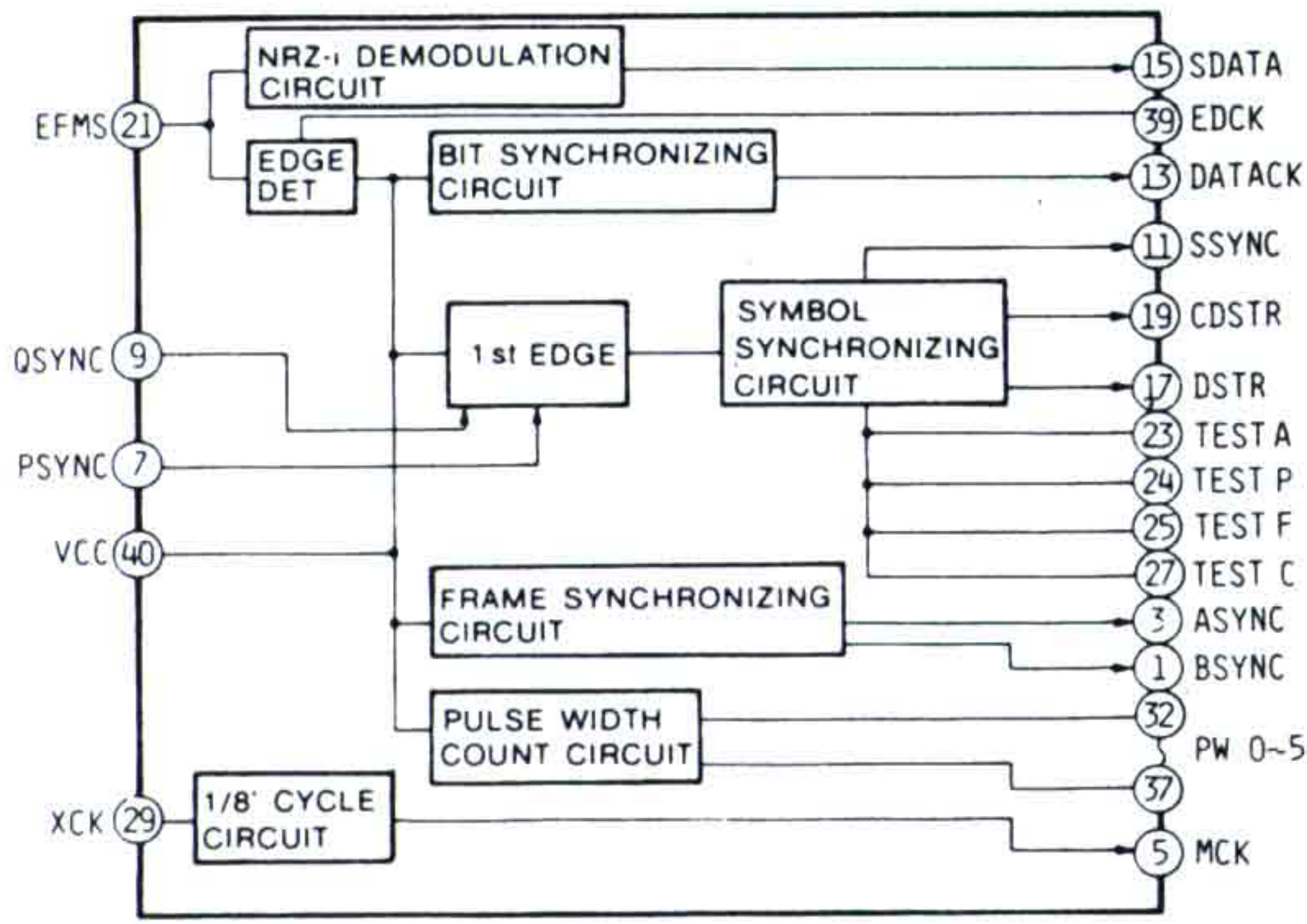
IC402(MB15529)
