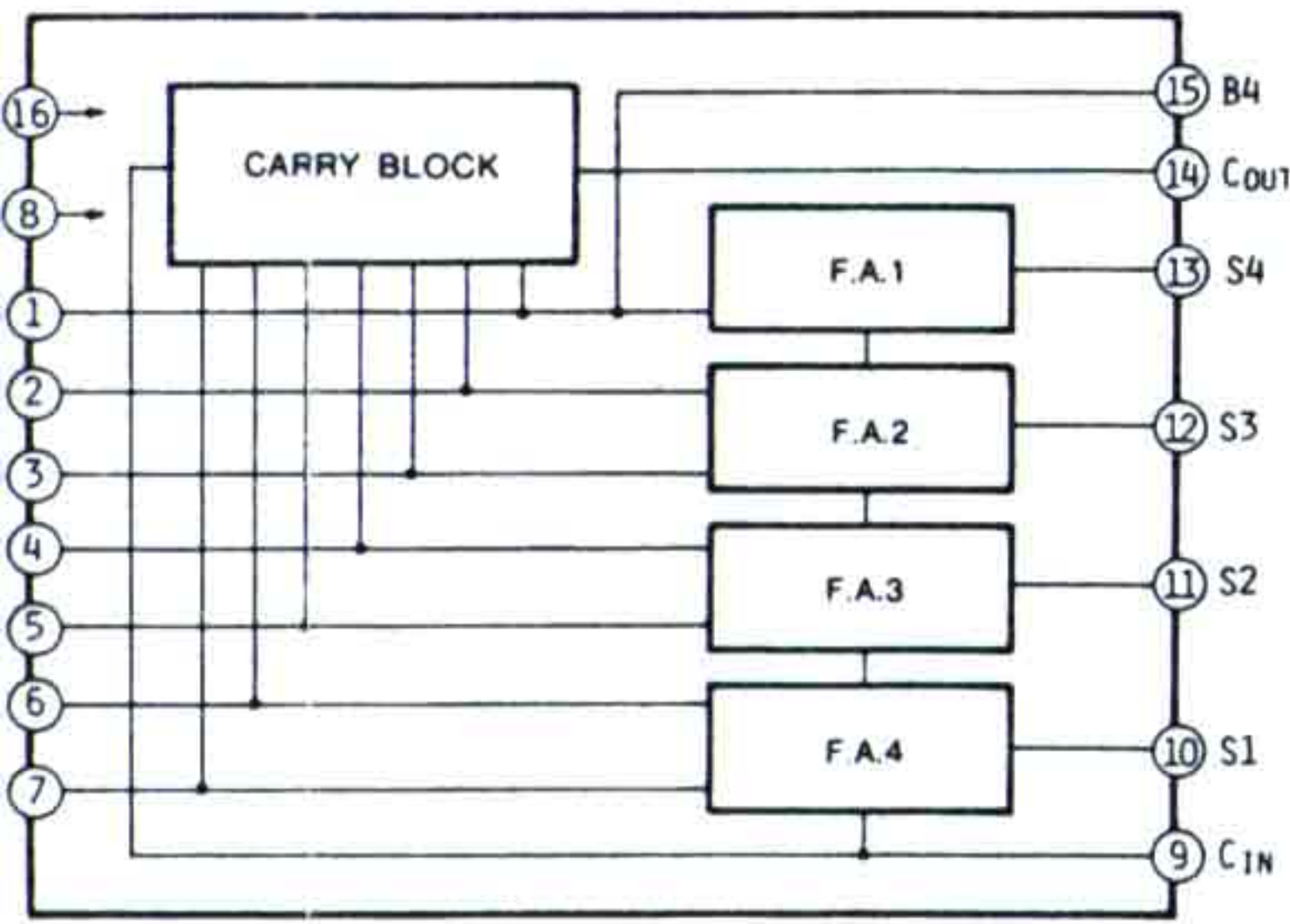
IC406, 407(TC4008BP)
