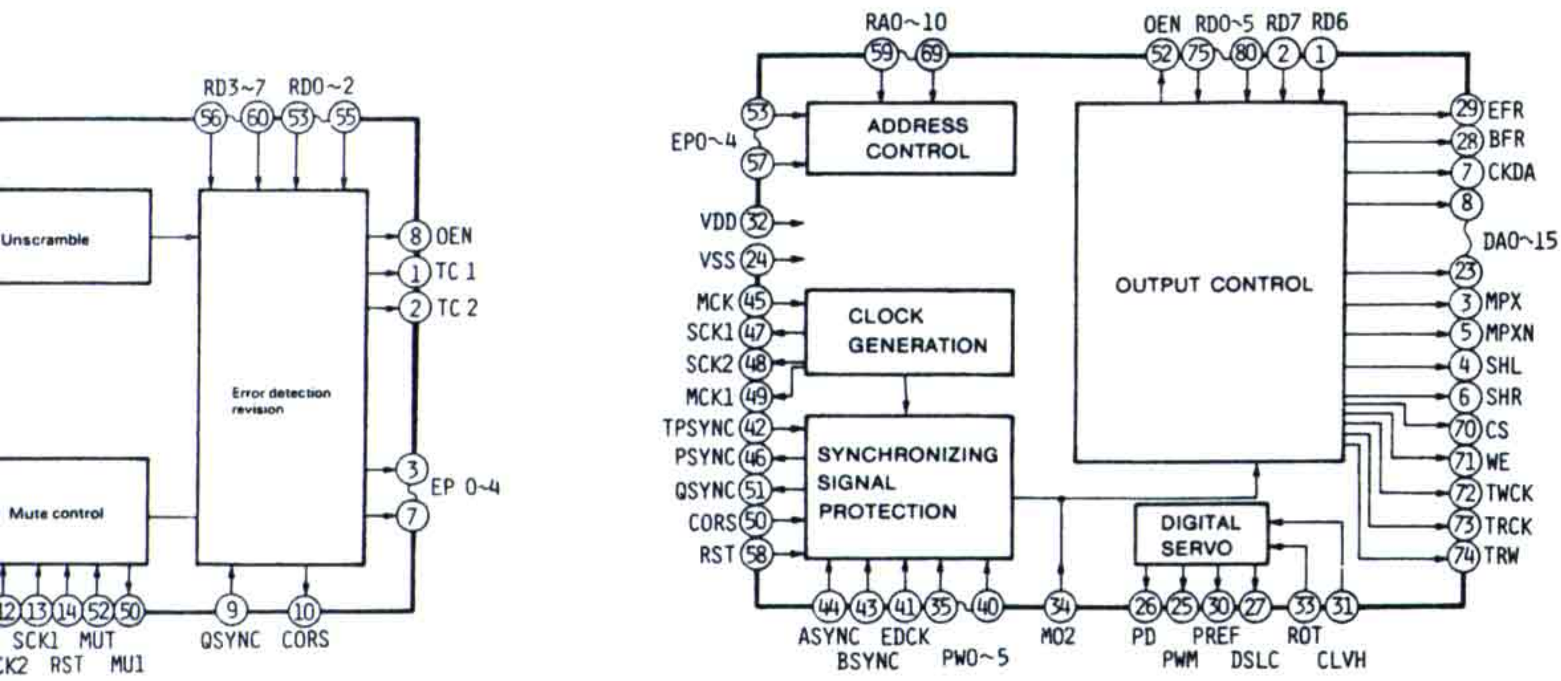
IC404(HD61902)
