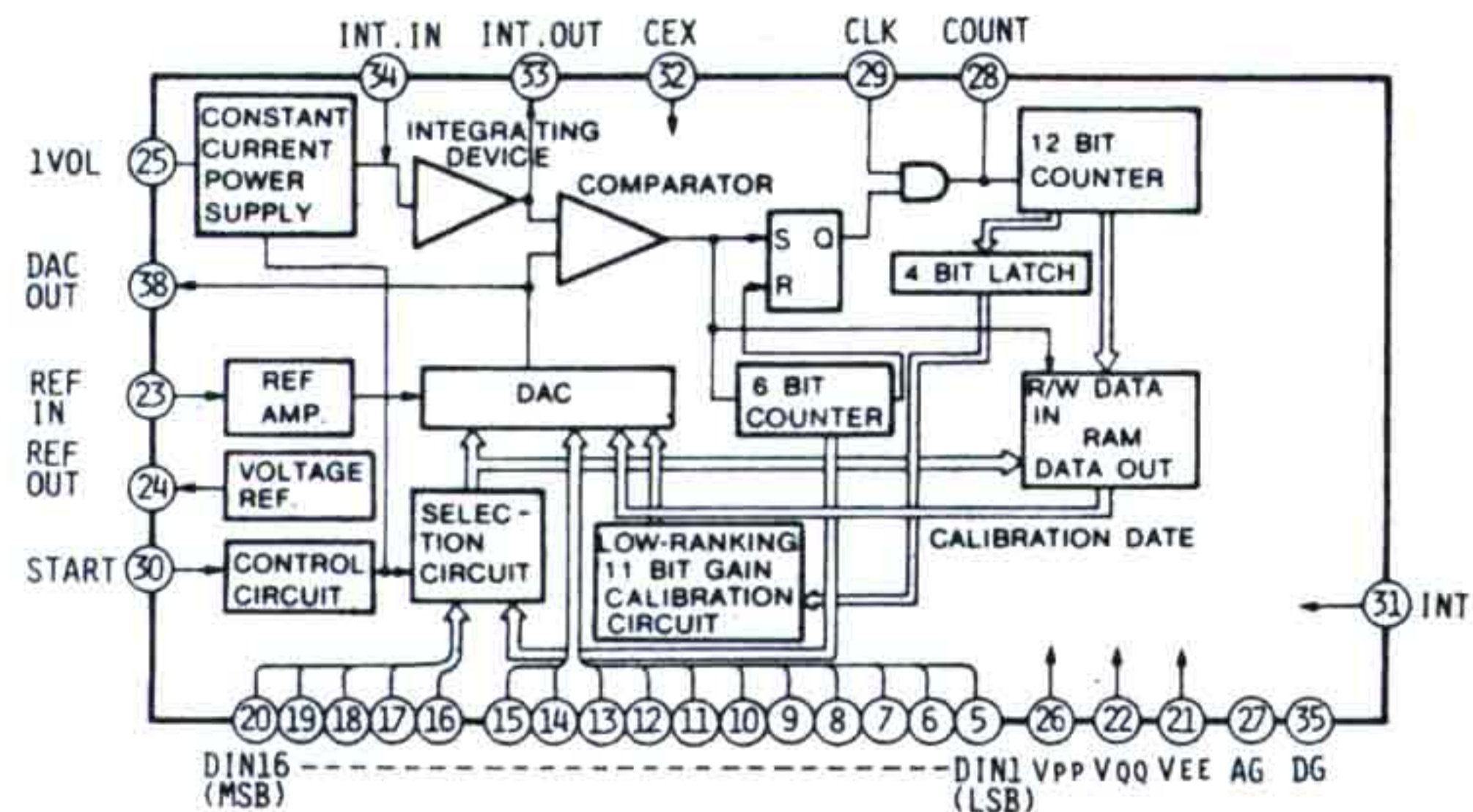
IC410(HA16633)
