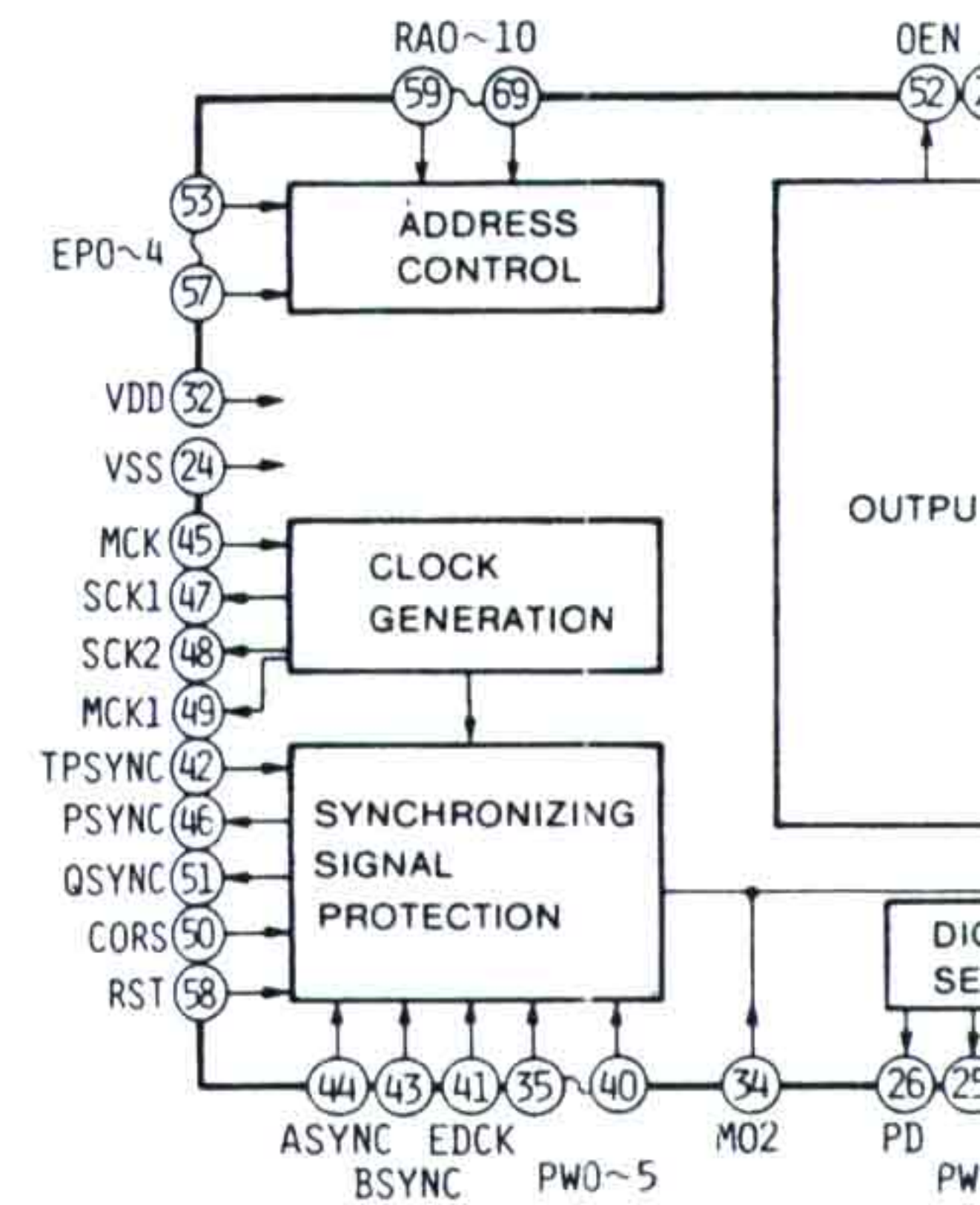
IC404(HD61902)
