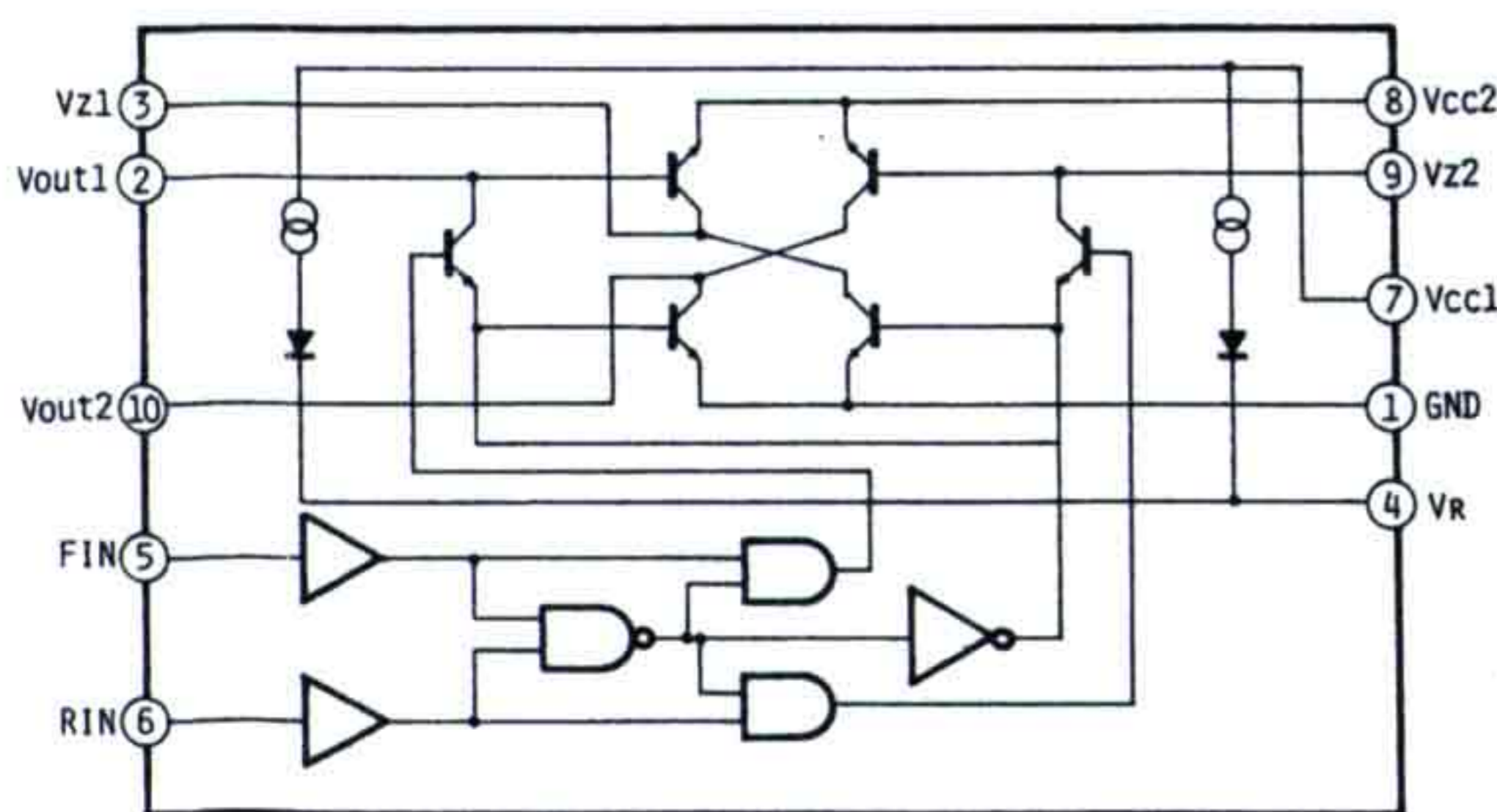
IC900(BA6109)
