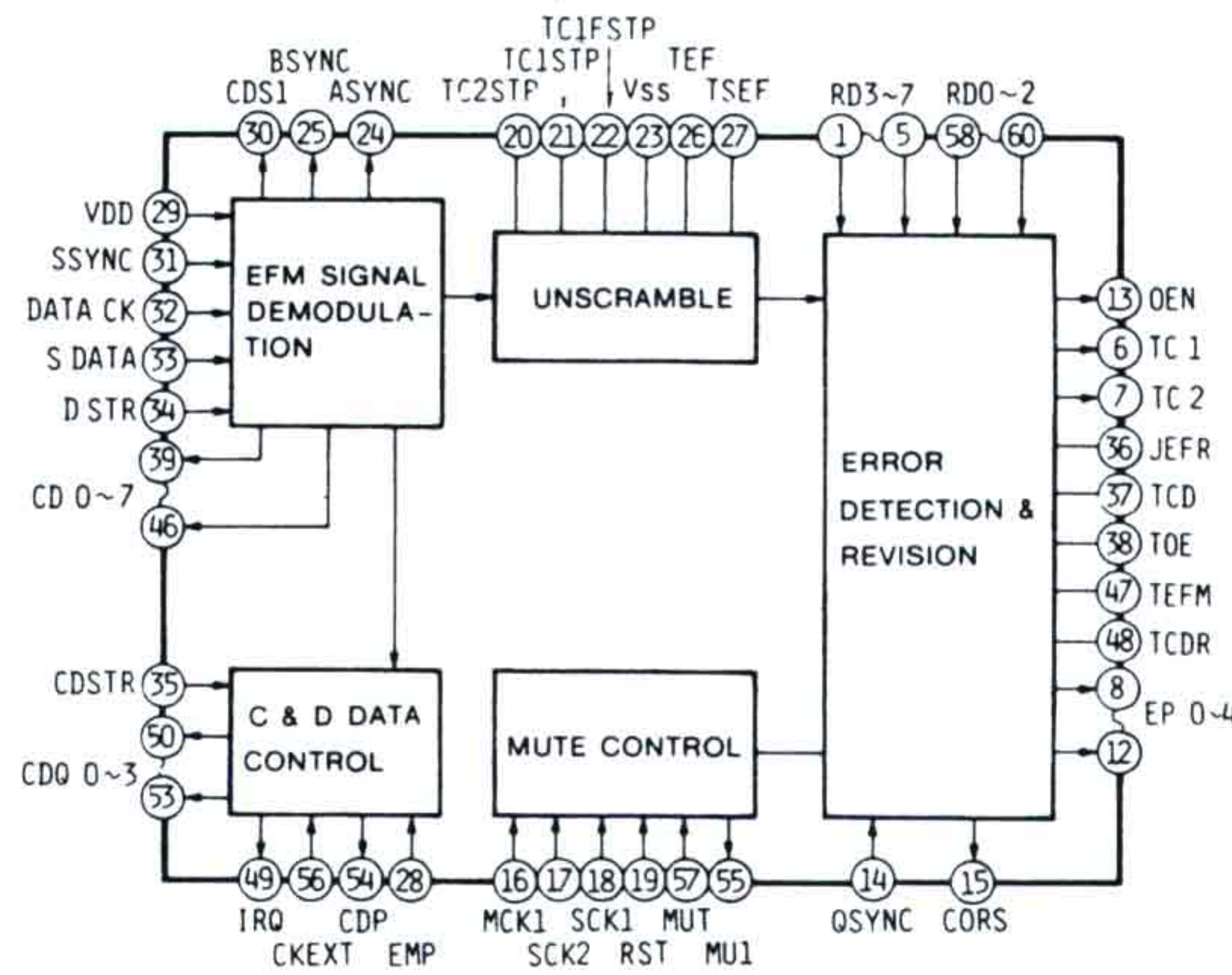
IC403(HD61901)
