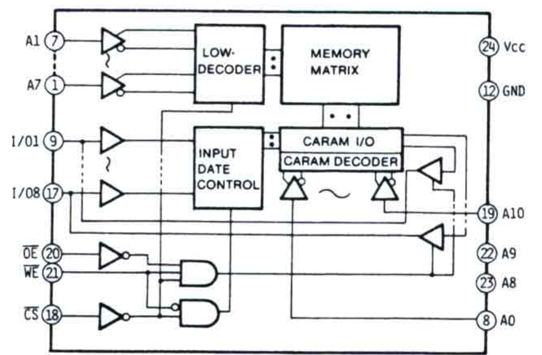
IC405(HM6116P-4)
