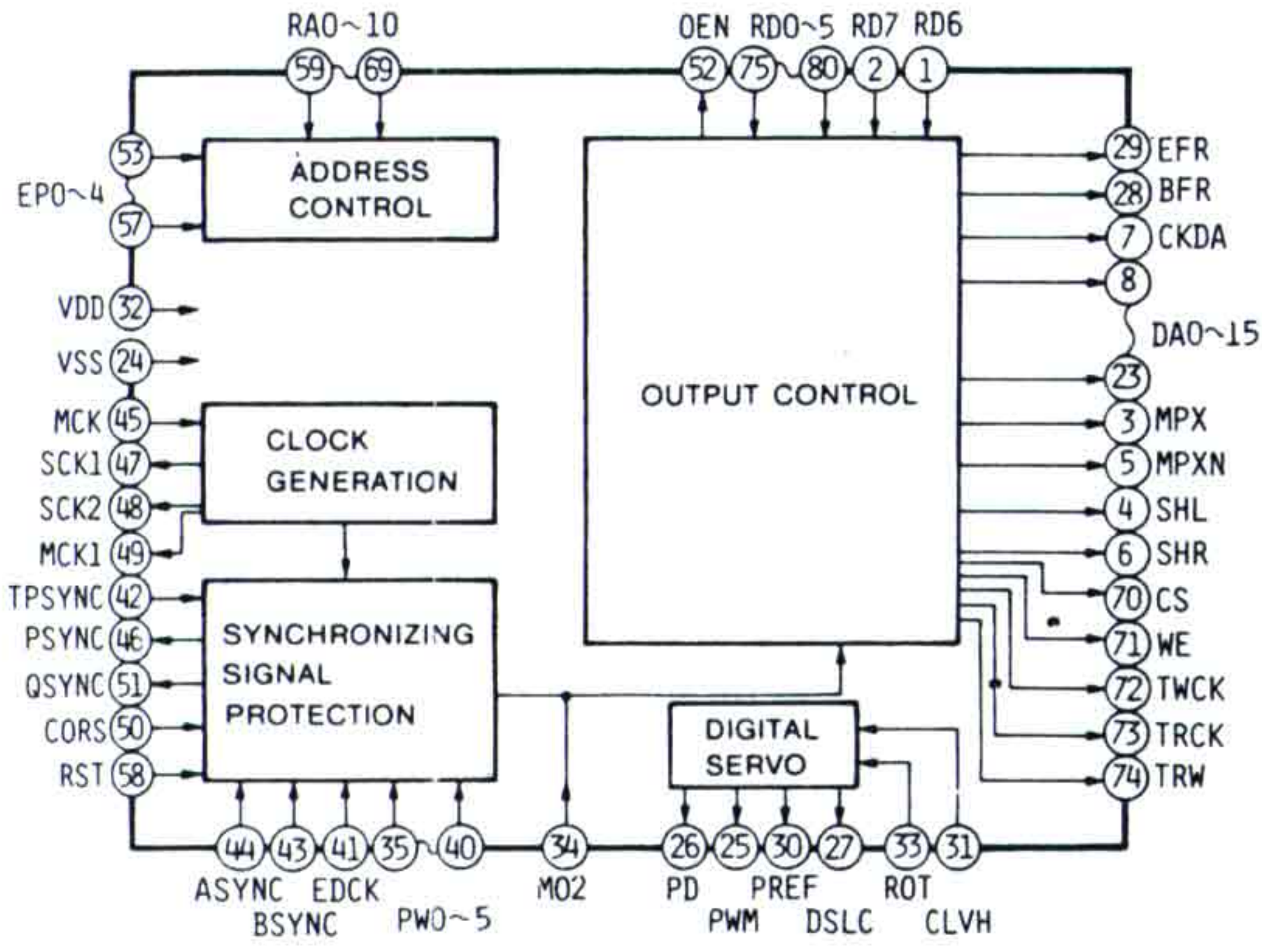
IC404(HD61902)
