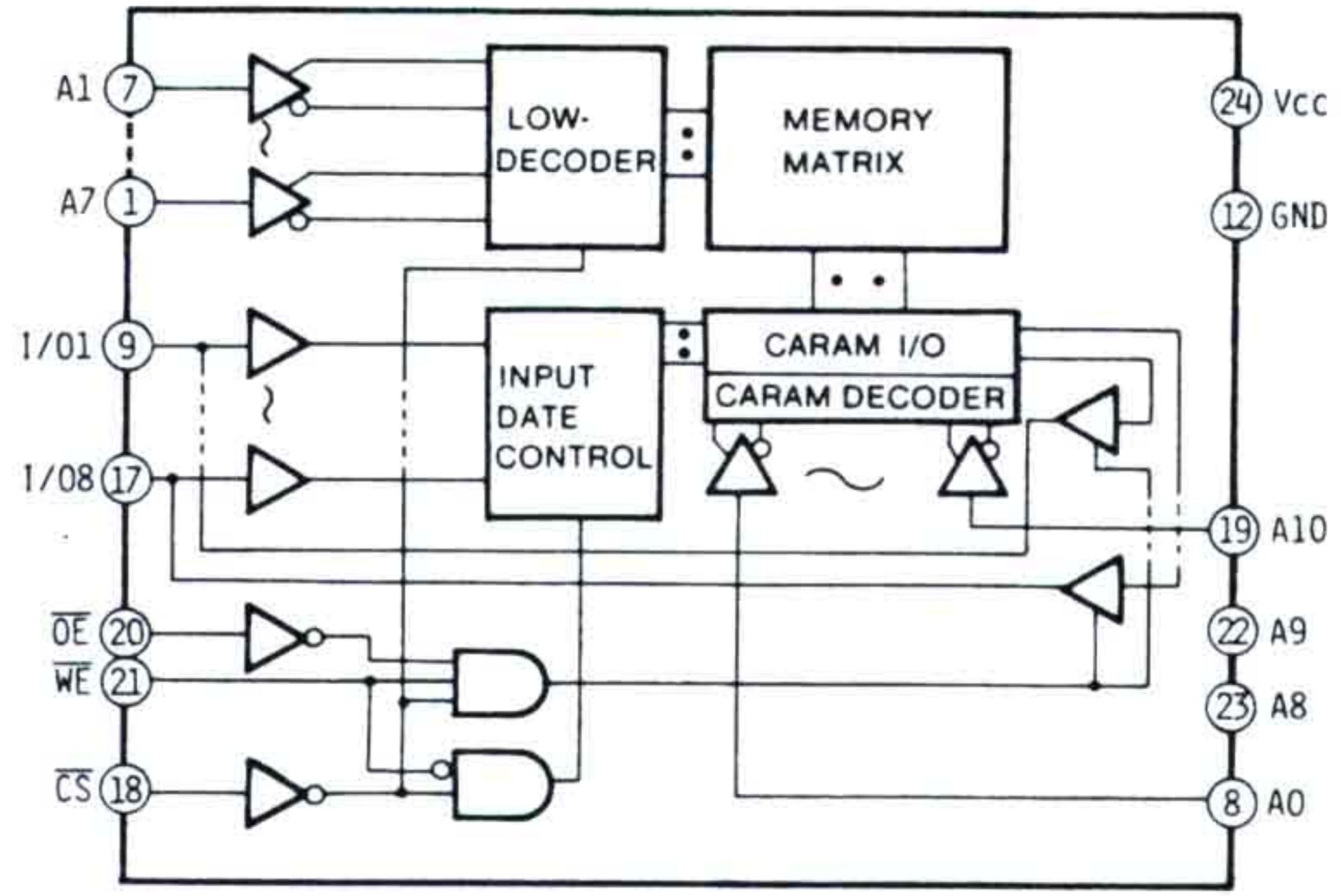
IC405(HM6116P-4)
