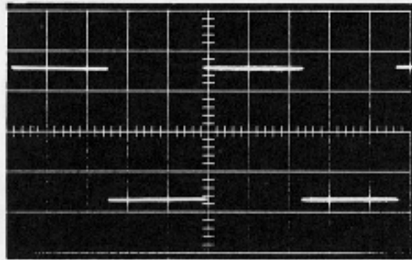
100 Hz, 200 watts protective rolloff removed
