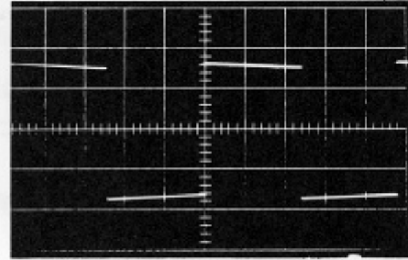
20 Hz, 200 watts protective rolloff removed
