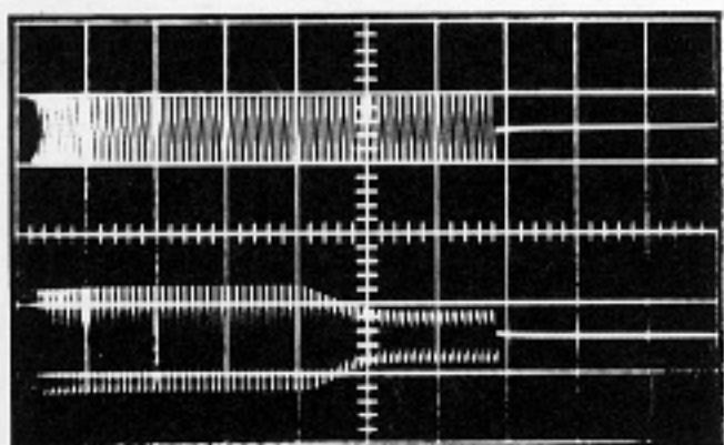
1 second 50 watt drive / Dynaguard-20 40 Hz 200 ms/cm
