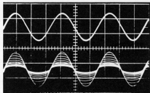
Onset of Dynaguard-20 on 200 watt signal 150 Hz
