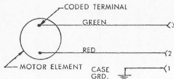
WIRING DIAGRAM
