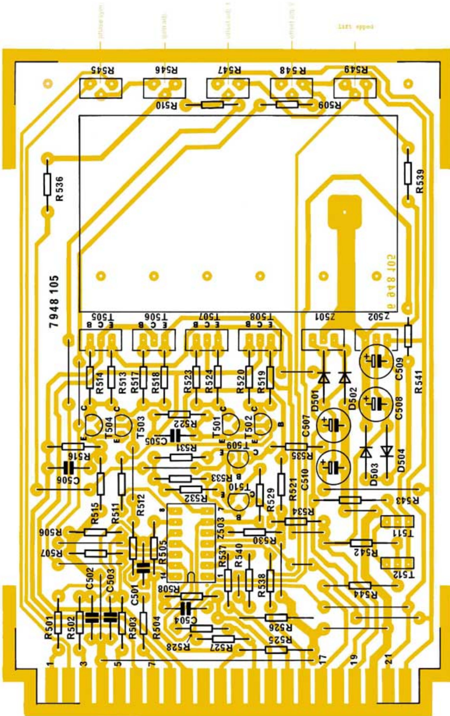
EMT 948 Endstufen-Platine SERVO AMPLIFIER
