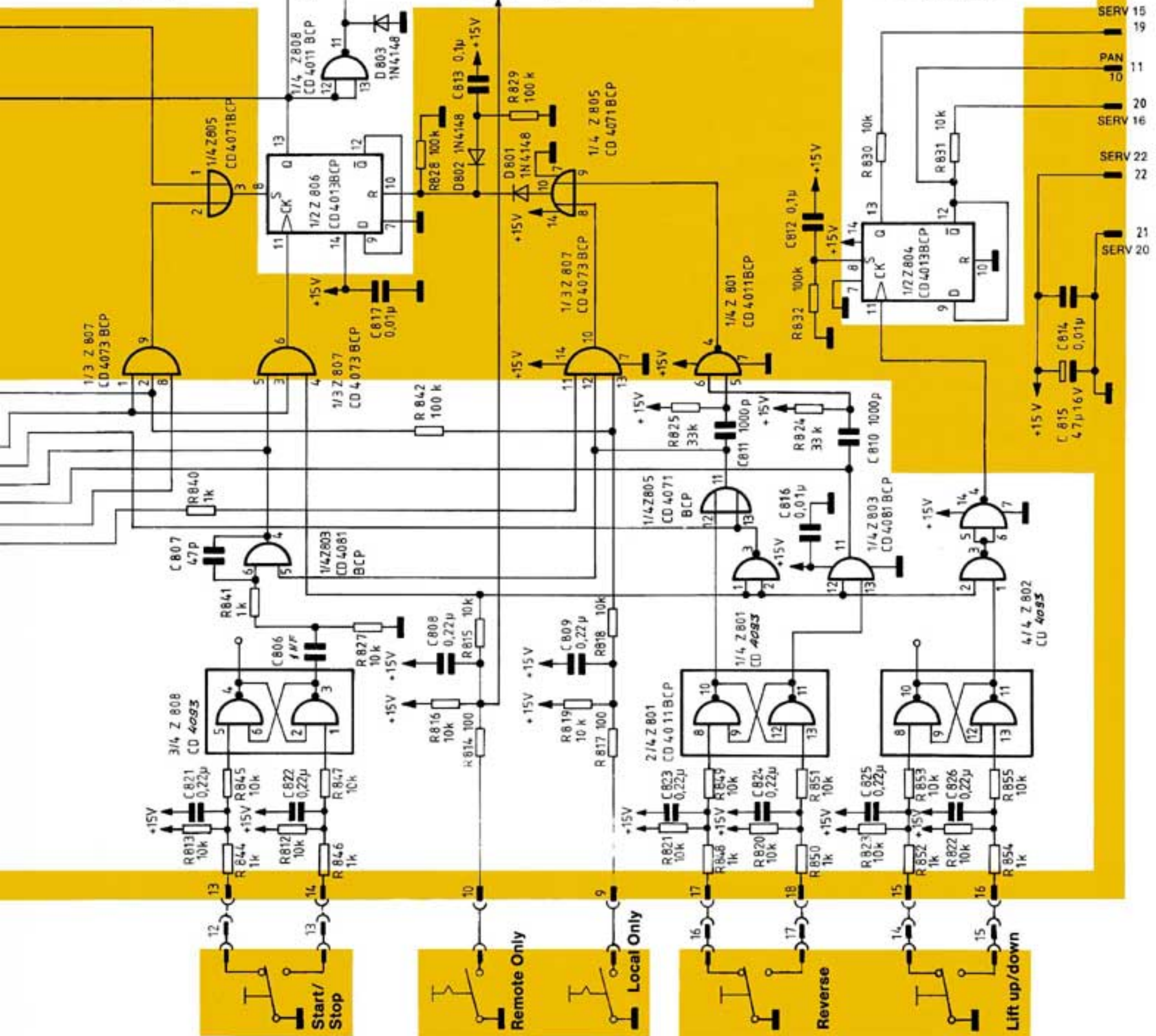
Control panel
