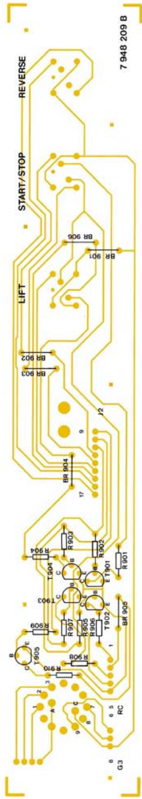
EMT 948 Tastenfeld 7 948 209 PUSH BUTTON BOARD
