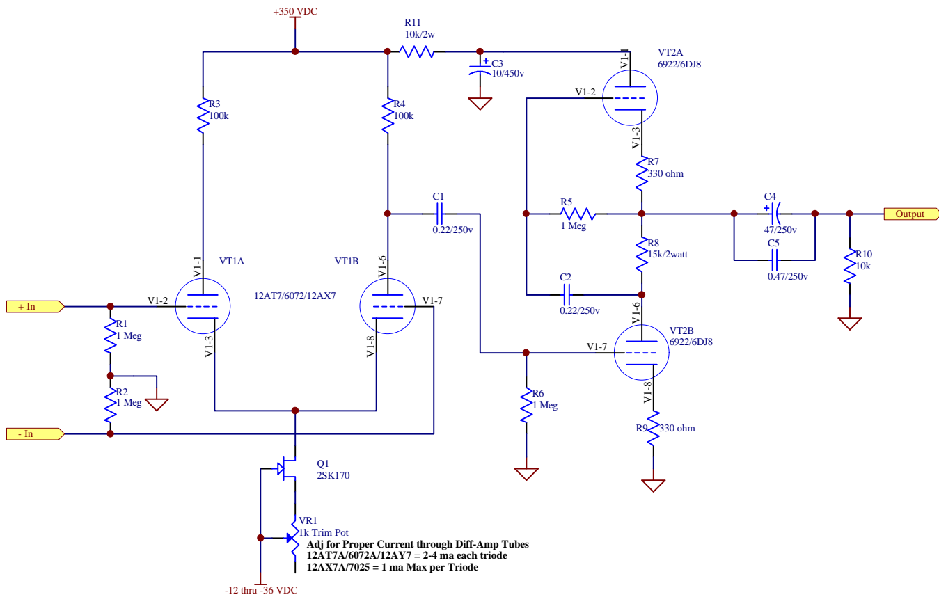
Forsell Technologies Vacuum Tube Opamp Amp
