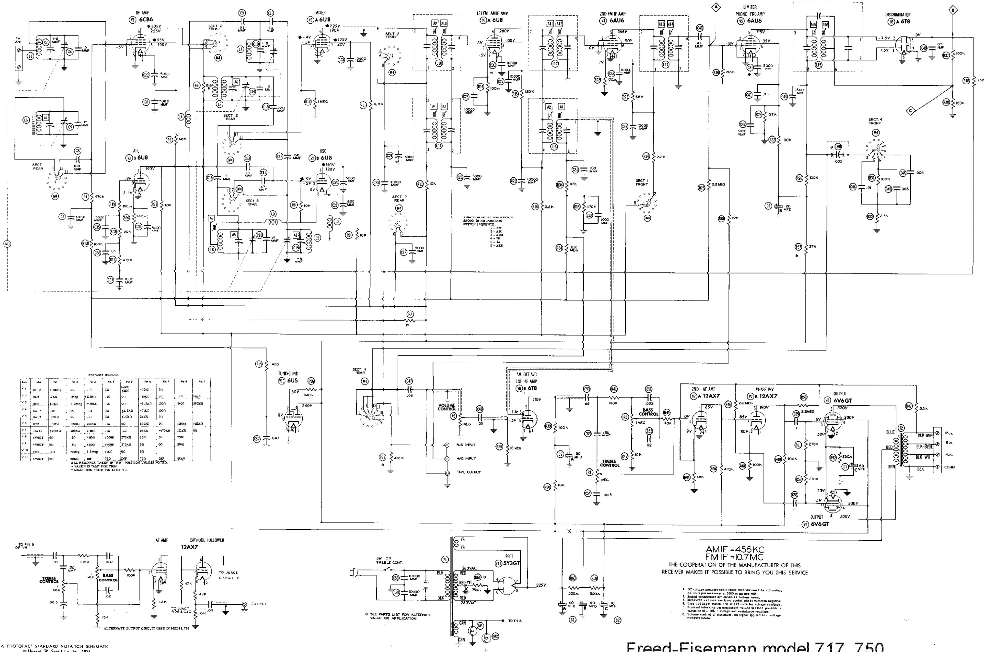
A PHOTOFACT STANDARD NOTATION SCHEMATIC © Howard W. Sams & Co., Inc. 1959
