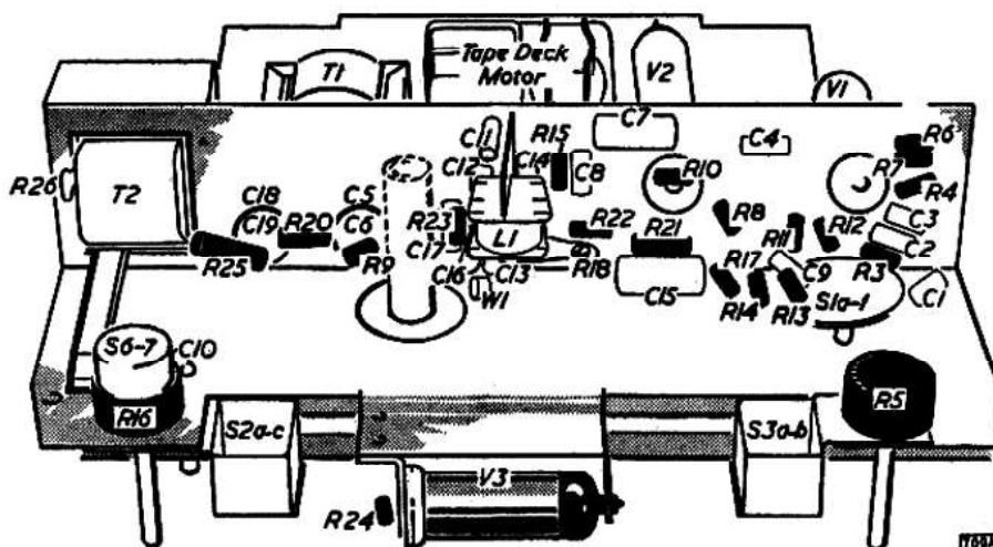
Chassis component layout.
