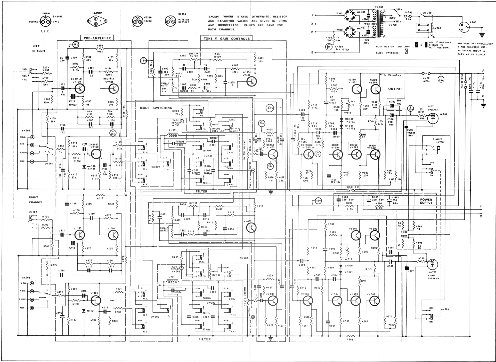
Circuit diagram of Ferrograph Integrated Stereo Amplifier F307 MK2
