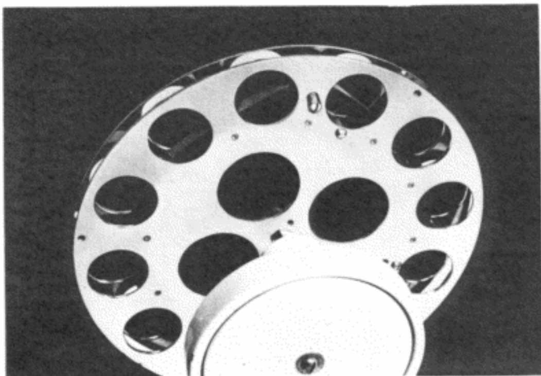
FIG. 5. LOADING OF LOOP CASSETTE
