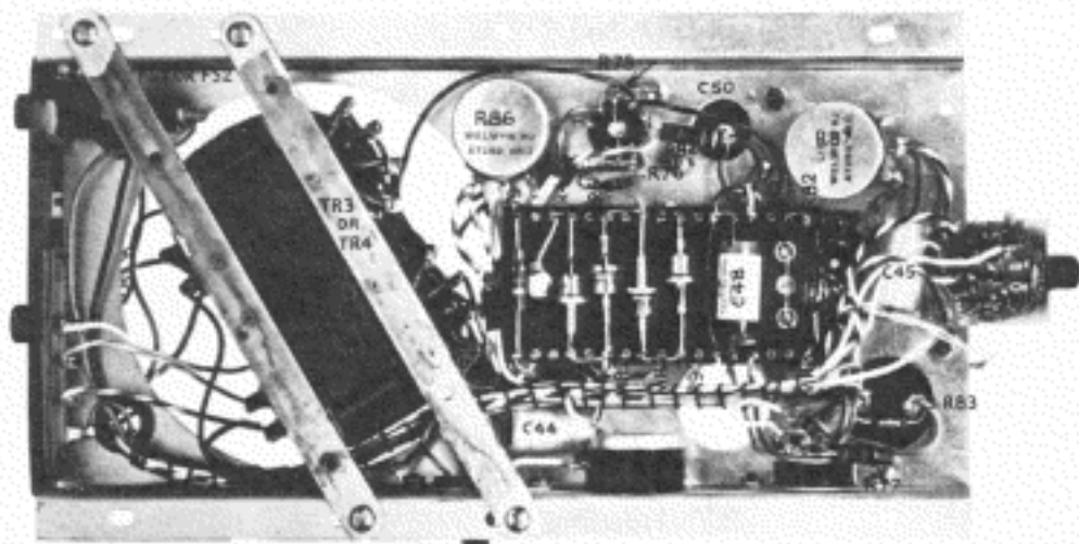
FIG. 8. POWER UNIT UNDERSIDE VIEW
