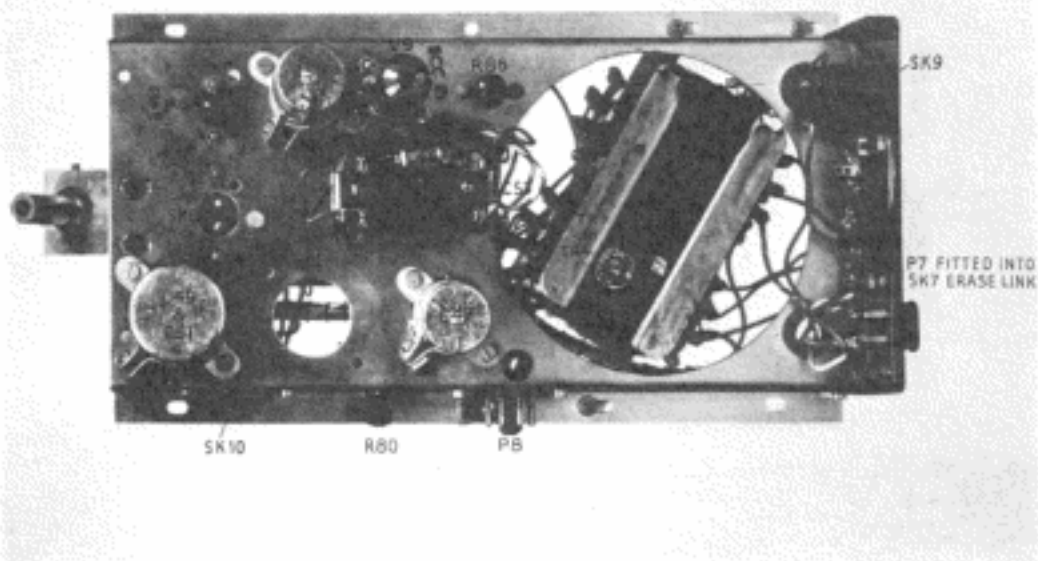
FIG. 9. POWER UNIT TOP VIEW
