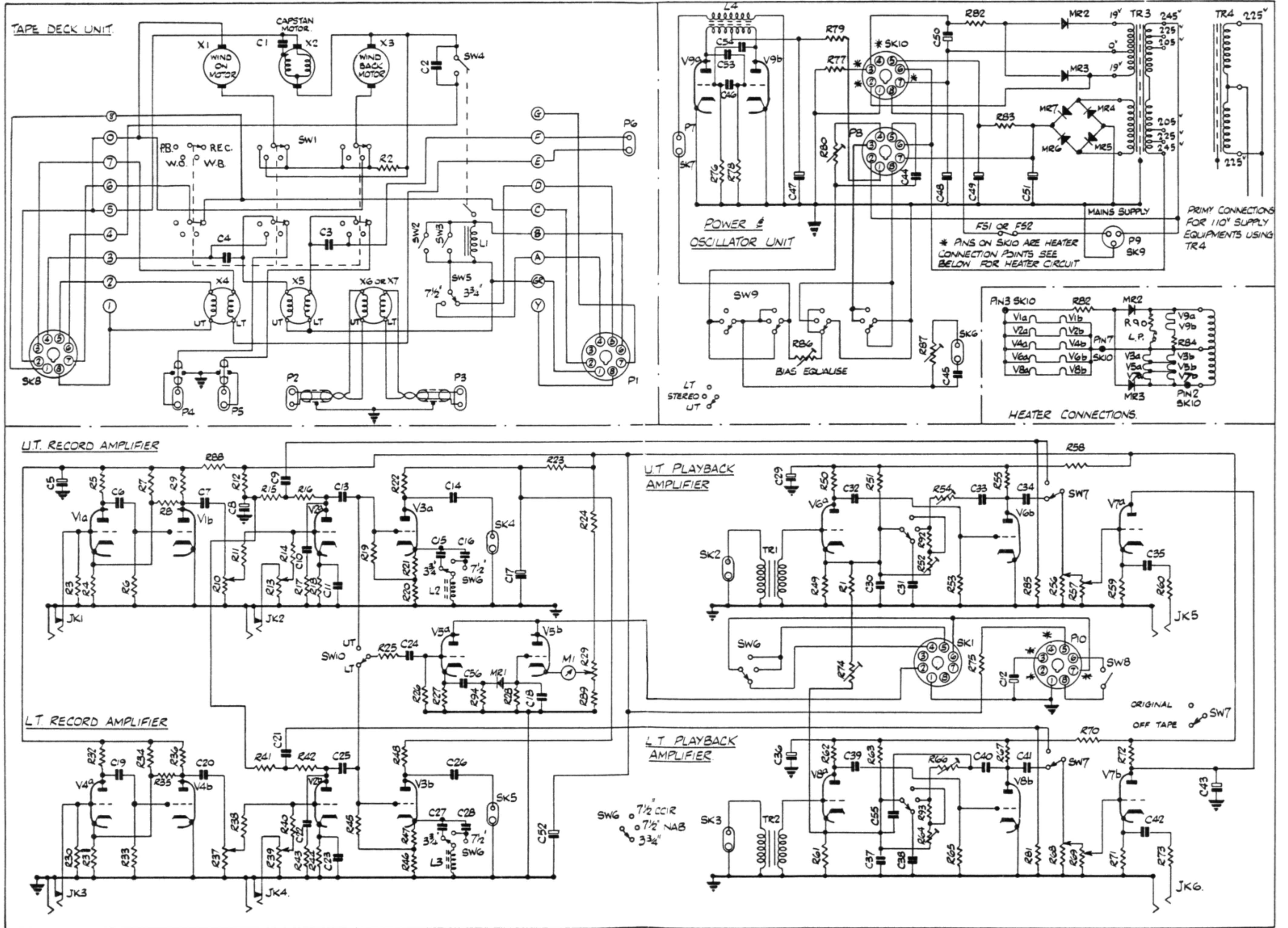
FIG. 16. COMPLETE CIRCUIT DIAGRAM, SERIES 420
