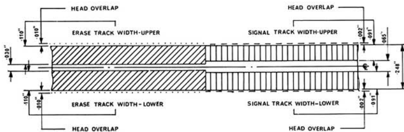
FIG. 24. STEREO TRACK DIMENSIONS MODELS 702 AND 722
