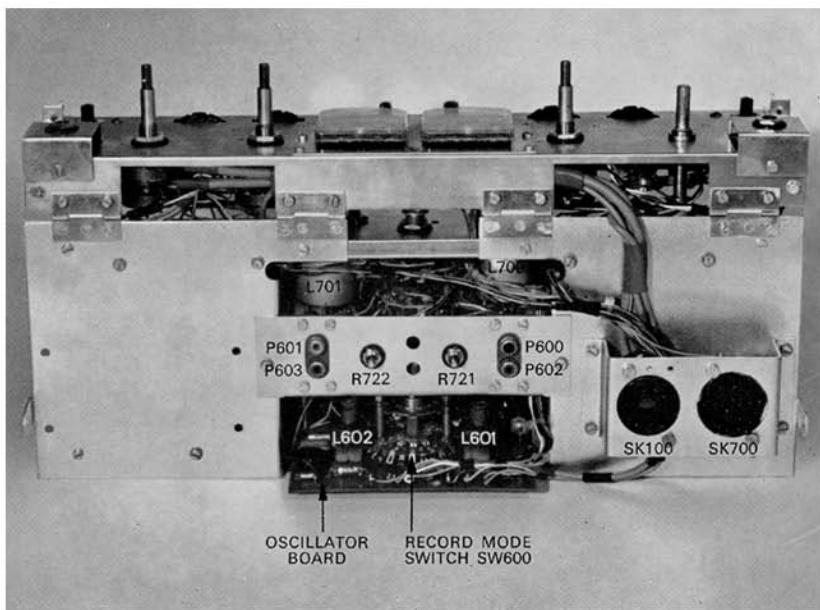
FIG. 29. STEREO AMPLIFIER REAR VIEW
