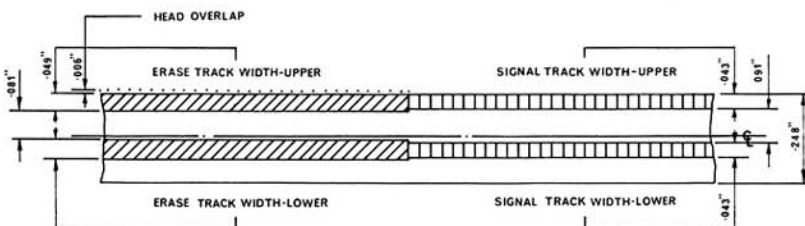
FIG. 25. STEREO TRACK DIMENSIONS MODELS 704 AND 724
