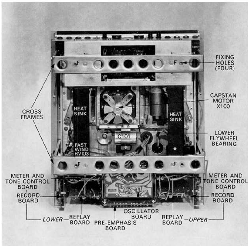
FIG. 14. RECORDER CHASSIS—REAR VIEW
