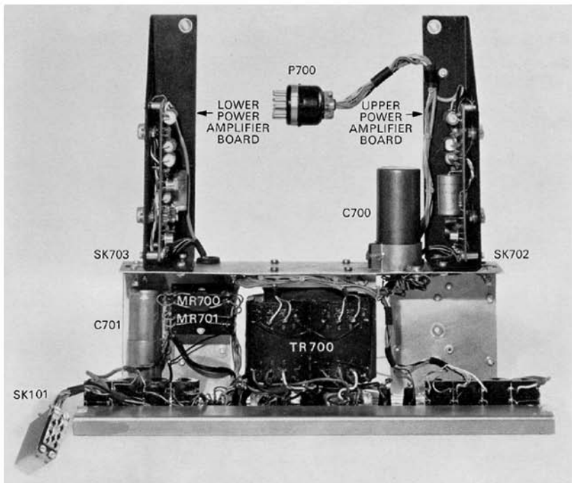
FIG. 31. STEREO POWER UNIT
