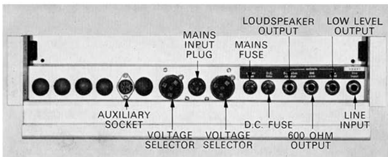
FIG. 3. REAR PANEL—MONO
