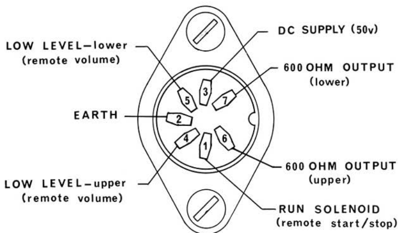
FIG. 12. AUXILIARY SOCKET CONNECTIONS
