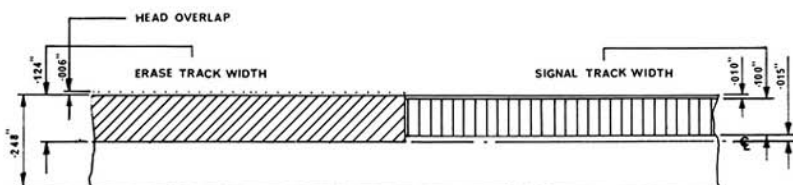
FIG. 21. MONO TRACK DIMENSIONS MODEL 713
