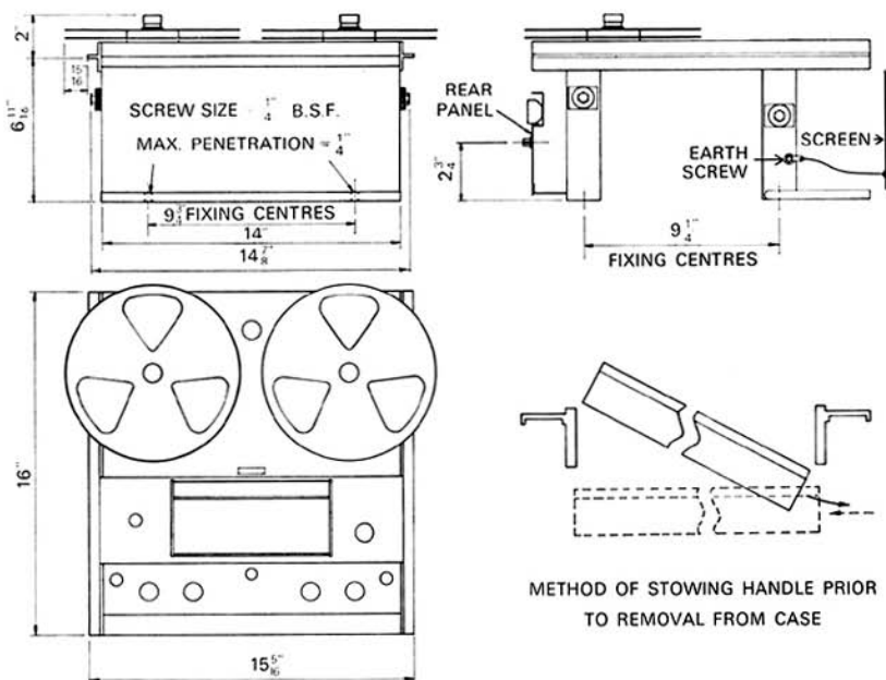
FIG. 15. CHASSIS MODEL DIMENSIONS
