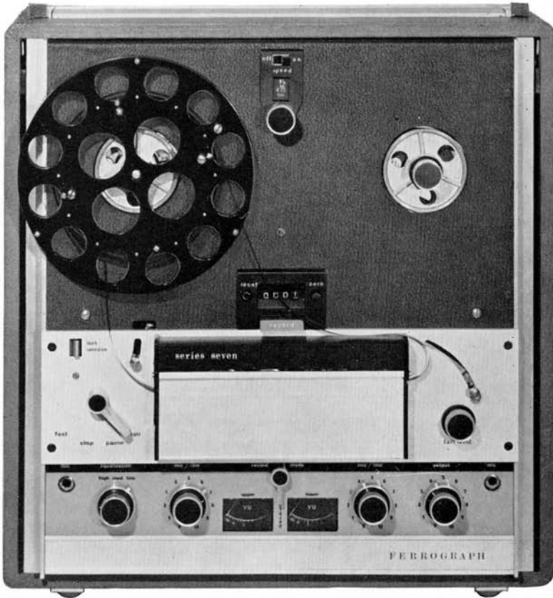
FIG. 19. ENDLESS LOOP CASSETTE
