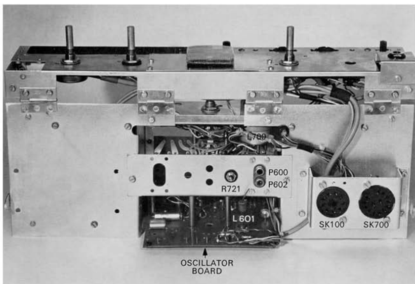
FIG. 27. MONO AMPLIFIER REAR VIEW
