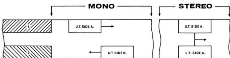
FIG. 9. TRACK DISPOSITIONS—HALF TRACK
