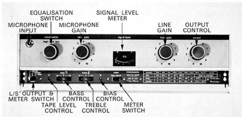
FIG. 7. AMPLIFIER CONTROLS—MONO
