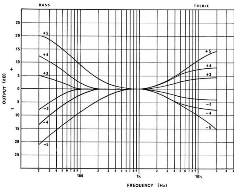
FIG. 18. EFFECT OF BASS AND TREBLE CONTROLS
