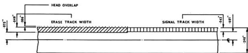
FIG. 23. MONO TRACK DIMENSIONS MODELS 704 AND 724
