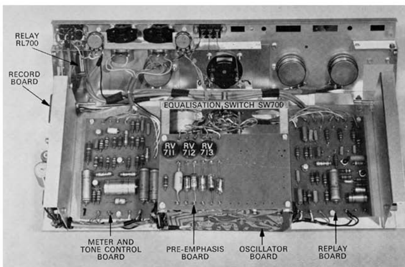
FIG. 26. MONO AMPLIFIER FRONT VIEW
