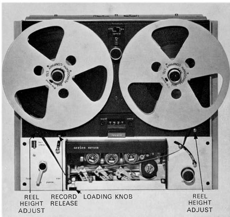
FIG. 5. TAPE LOADING
