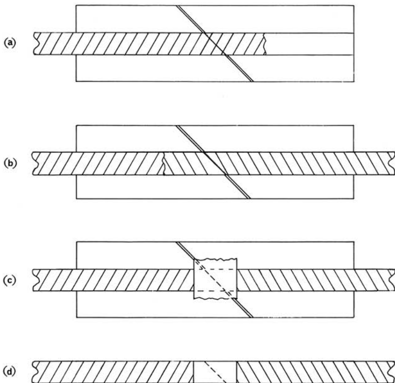
FIG. 11. TAPE SPLICING
