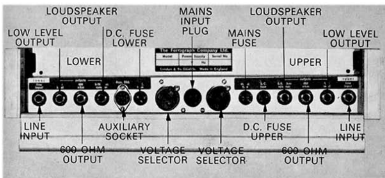
FIG. 4. REAR PANEL—STEREO
