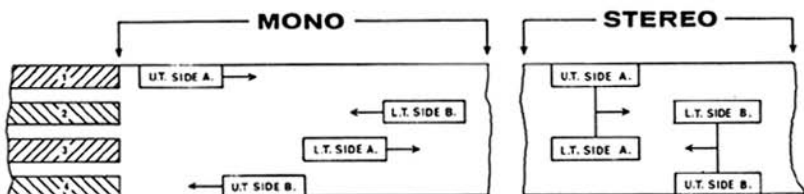
FIG. 10. TRACK DISPOSITIONS—QUARTER TRACK
