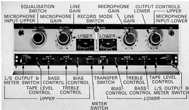
FIG. 8. AMPLIFIER CONTROLS—STEREO
