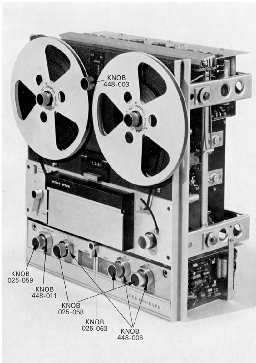
FIG. 17. RECORDER CHASSIS—FRONT VIEW
