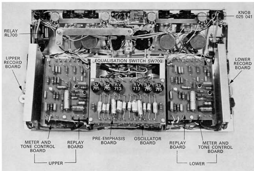
FIG. 28. STEREO AMPLIFIER FRONT VIEW
