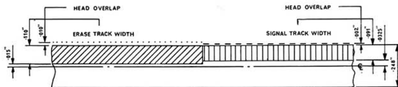
FIG. 22. MONO TRACK DIMENSIONS MODELS 702 AND 722
