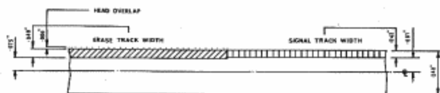
FIG. 23. MONO TRACK DIMENSIONS MODELS 704 AND 734
