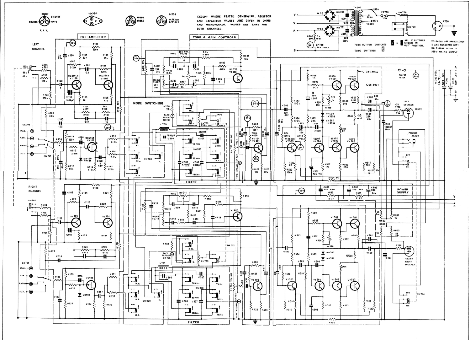
Circuit diagram of Ferrograph Integrated Stereo Amplifier F307 MK 2
