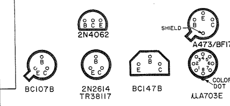
P2021 FM IF, AM IF, METER & MUTING AND MULTIPLEX
