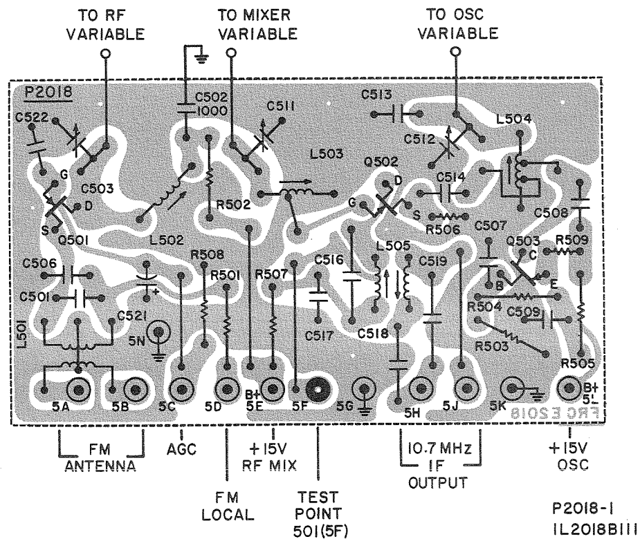
BOARD VIEWED FROM COMPONENT SIDE
