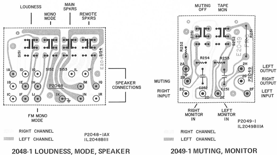
SCHEMATICS SHOWN ON MAIN CHASSIS DIAGRAM
