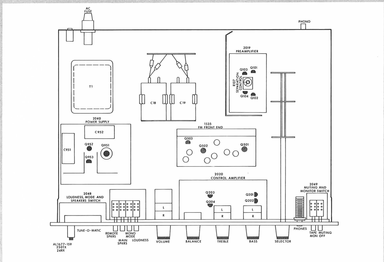
BOTTOM VIEW
