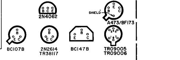
P2021-9-10 FM IF, AM IF, METER & MUTING AND MULTIPLEX
