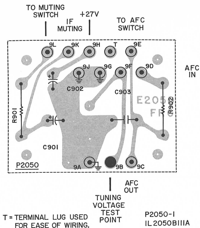
SCHEMATIC SHOWN ON MAIN CHASSIS DIAGRAM
