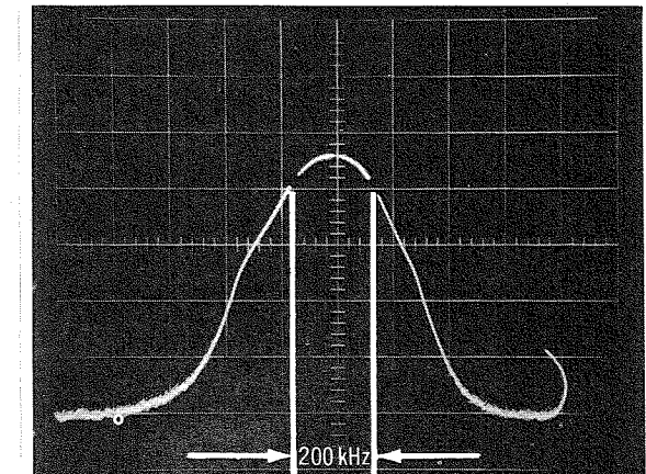
FM IF-LIMITED
