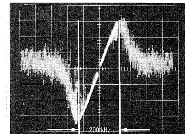
FM DETECTOR
