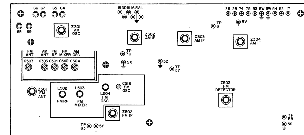
FM-AM TUNER BOARD LAYOUT
