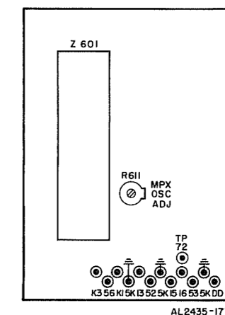
FM-AM TUNER BOARD LAYOUT
