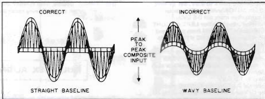
Figure 13. Composite Input To Multiplex Decoder
