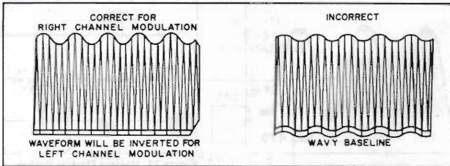
Figure 12. Waveform At Test Point 402
