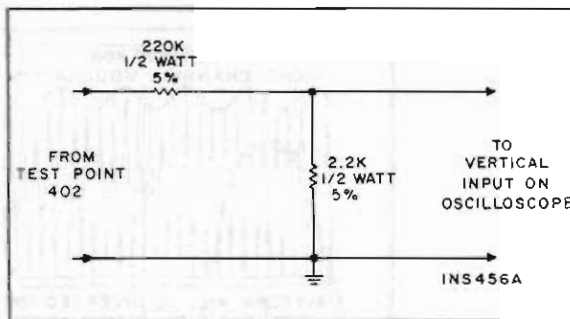
Figure 11. Voltage Divider Probe.
