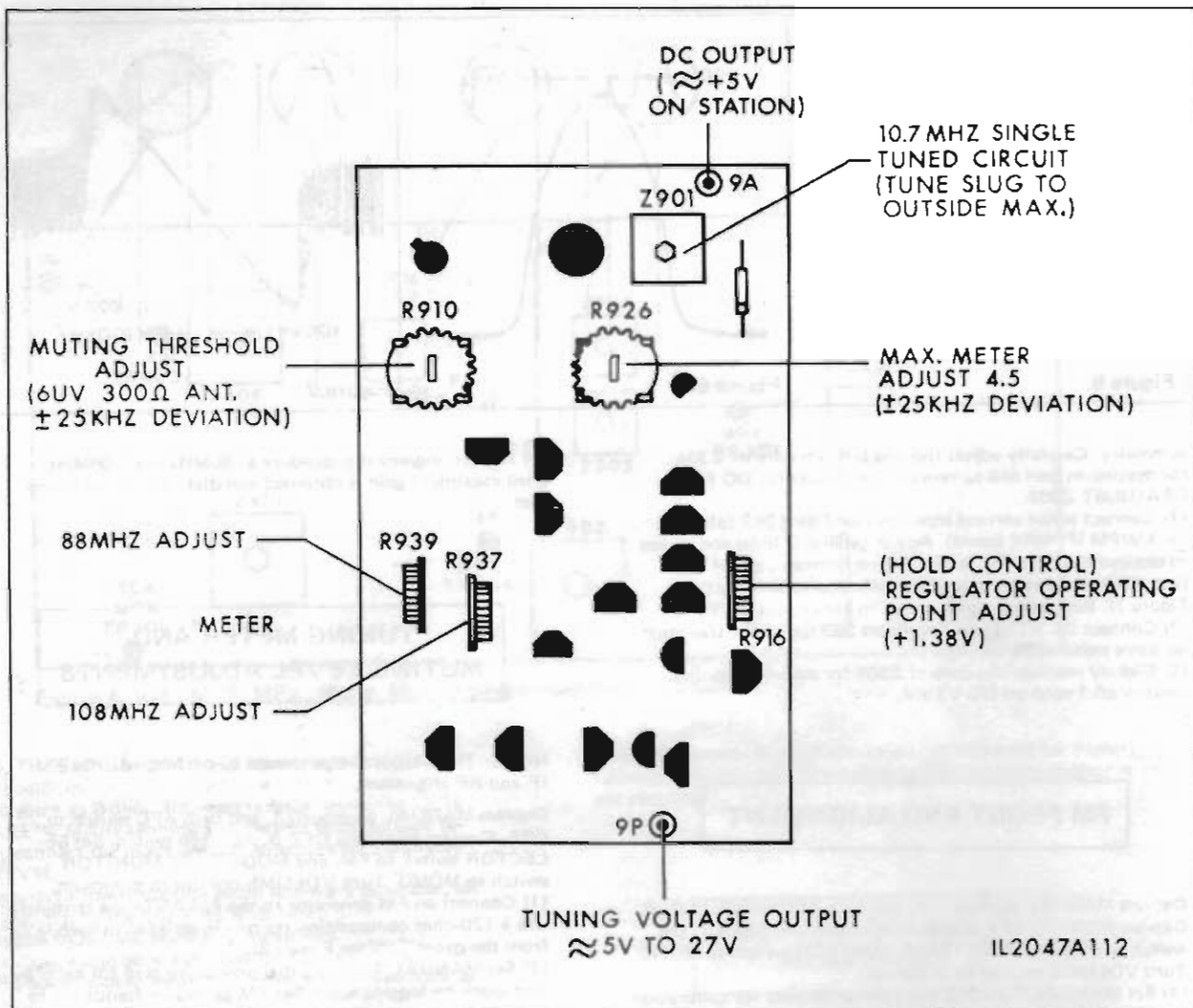
Figure 9. AUTOSCAN Board Alignment Location.
