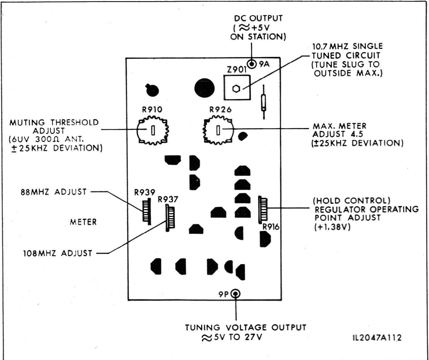
Figure 9. AUTOSCAN Board Alignment Location.
