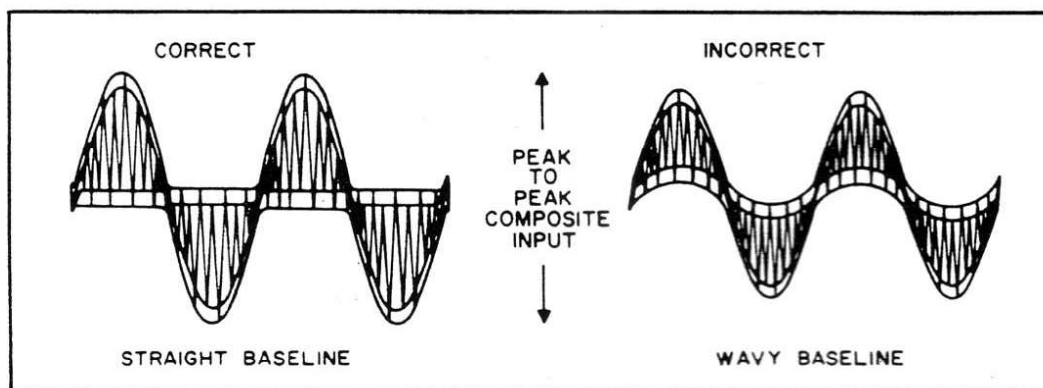
Figure 13. Composite Input To Multiplex Decoder
