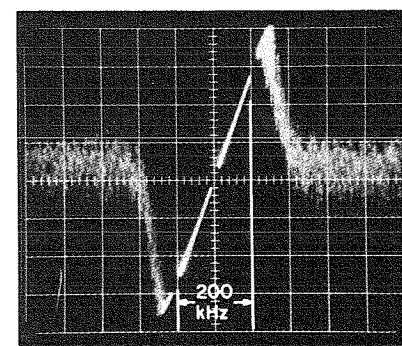
FM DETECTOR
