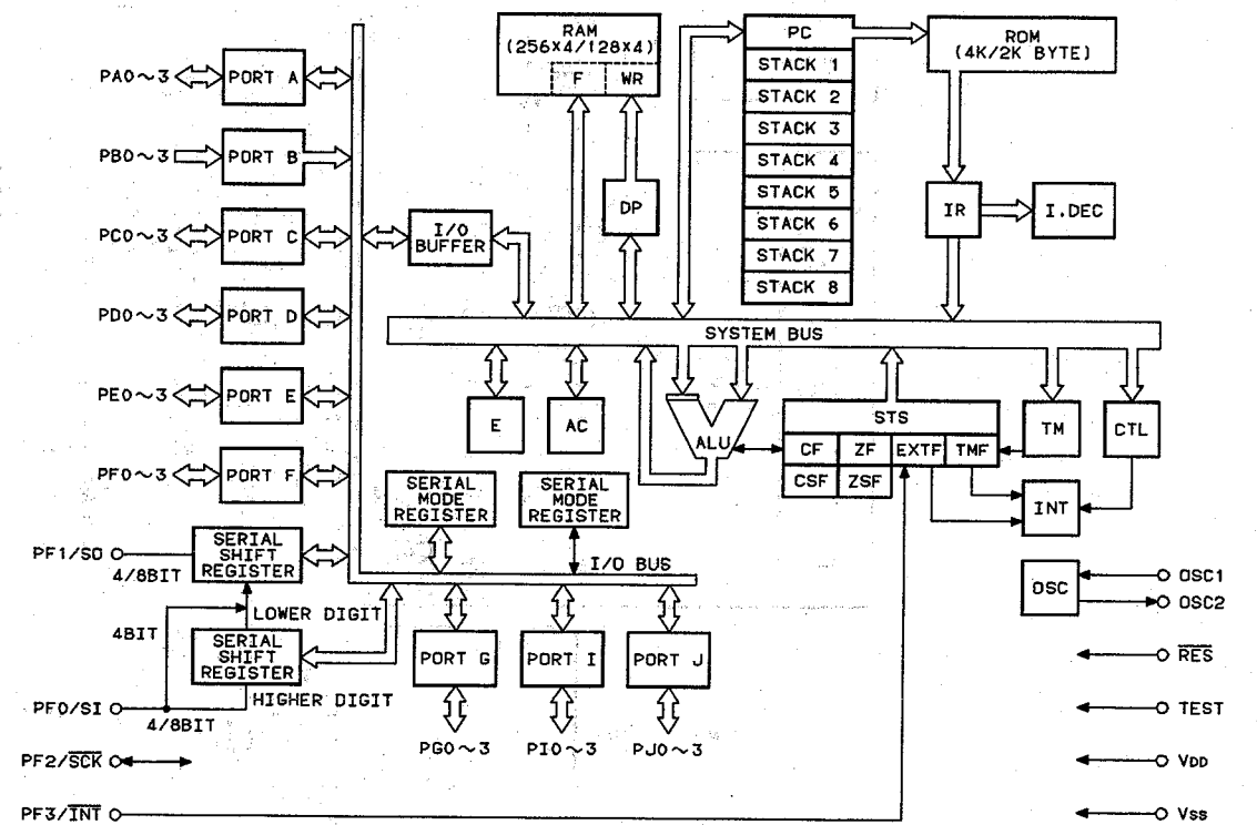
LC 6522H BLOCK DIAGRAM
