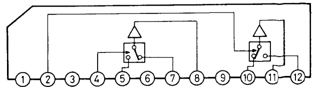
IC480 LA7222(AV SWITCH)
