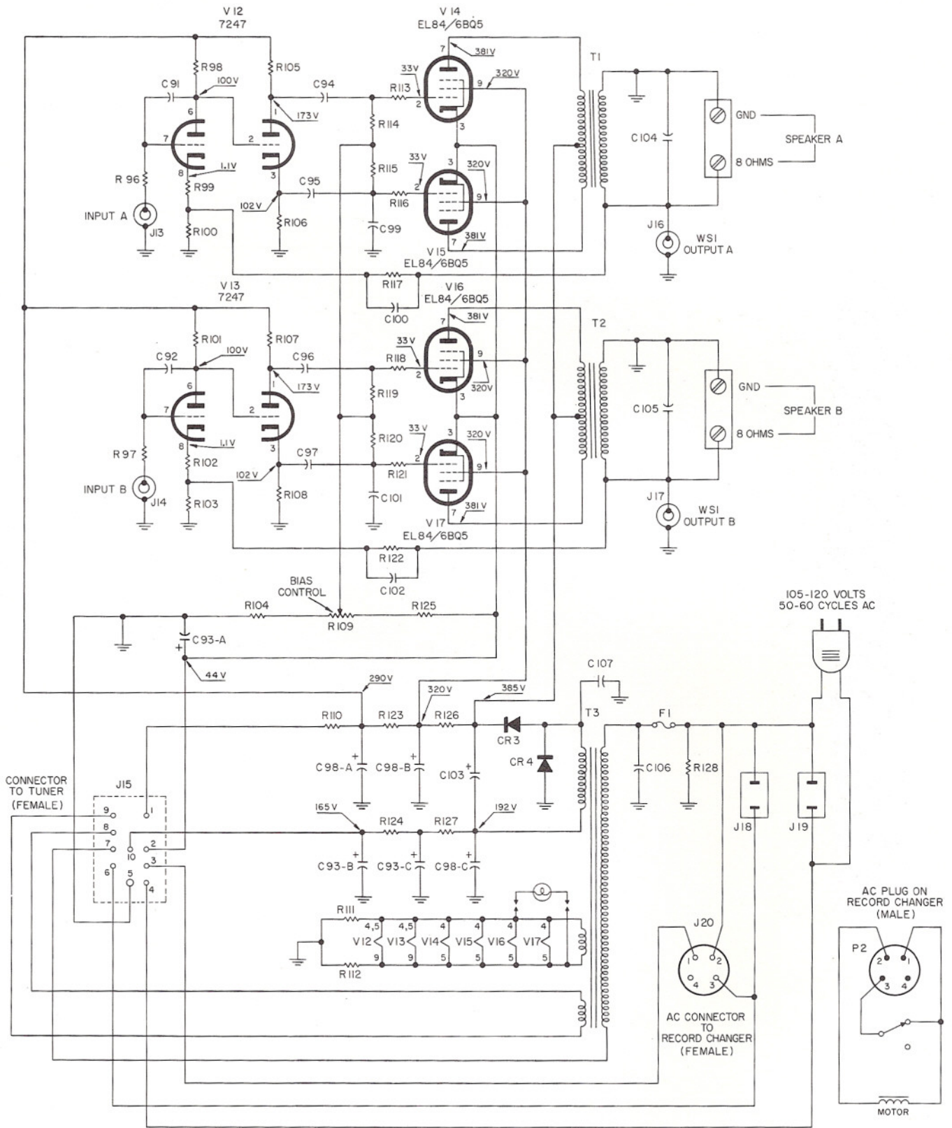
AW # 1896 P905-SCHEMATIC
