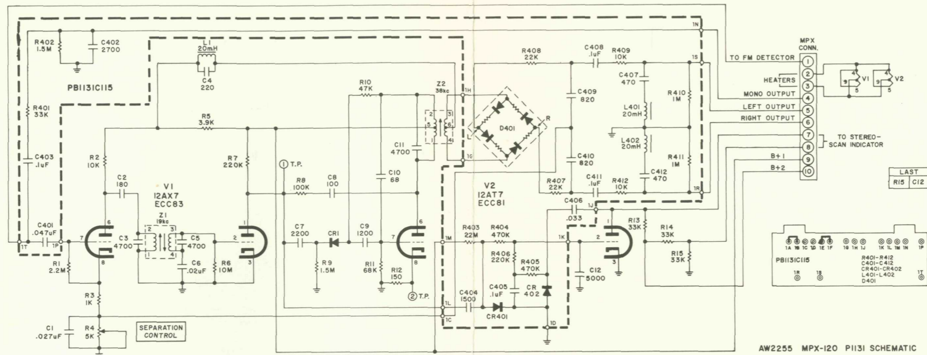
AW2255 MPX-120 P131 SCHEMATIC
