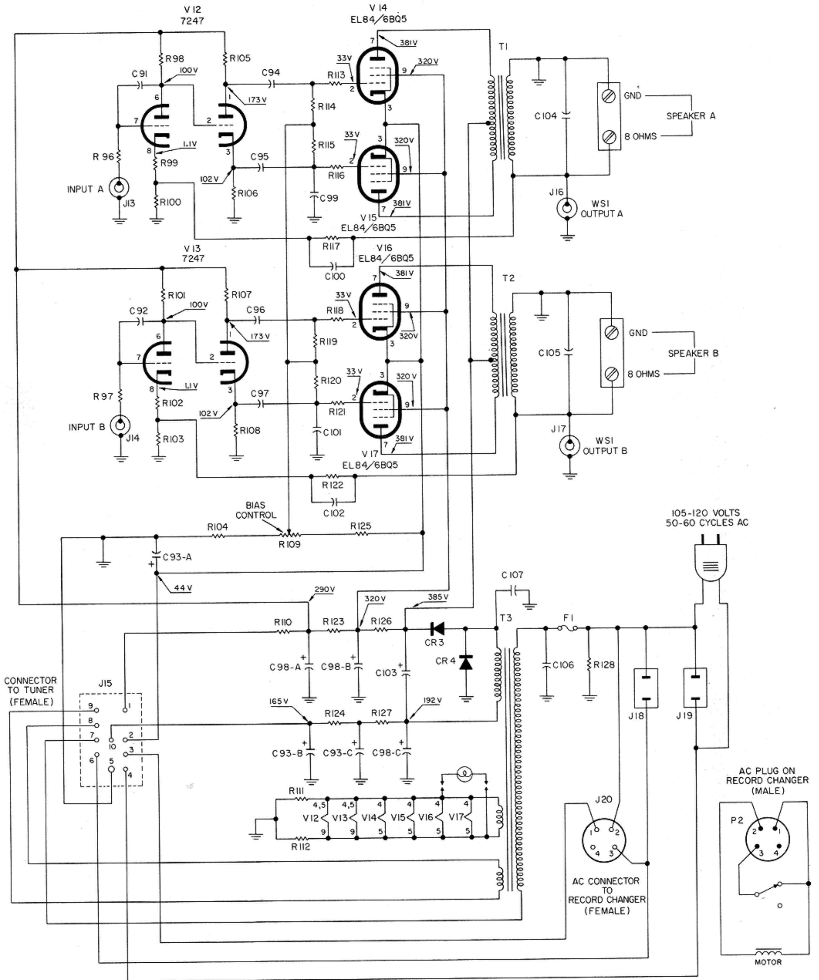
AW# 1896 P905-SCHEMATIC
