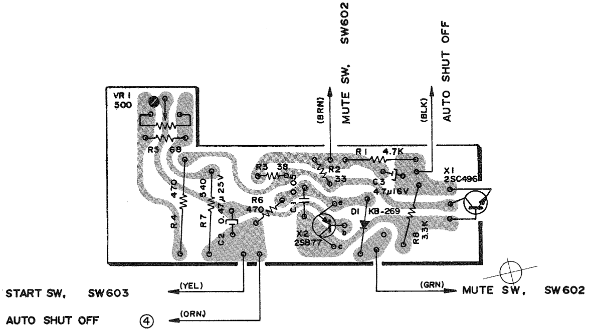
MOTOR GOVERNOR BOARD
