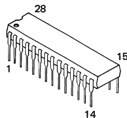
• TD6301P
